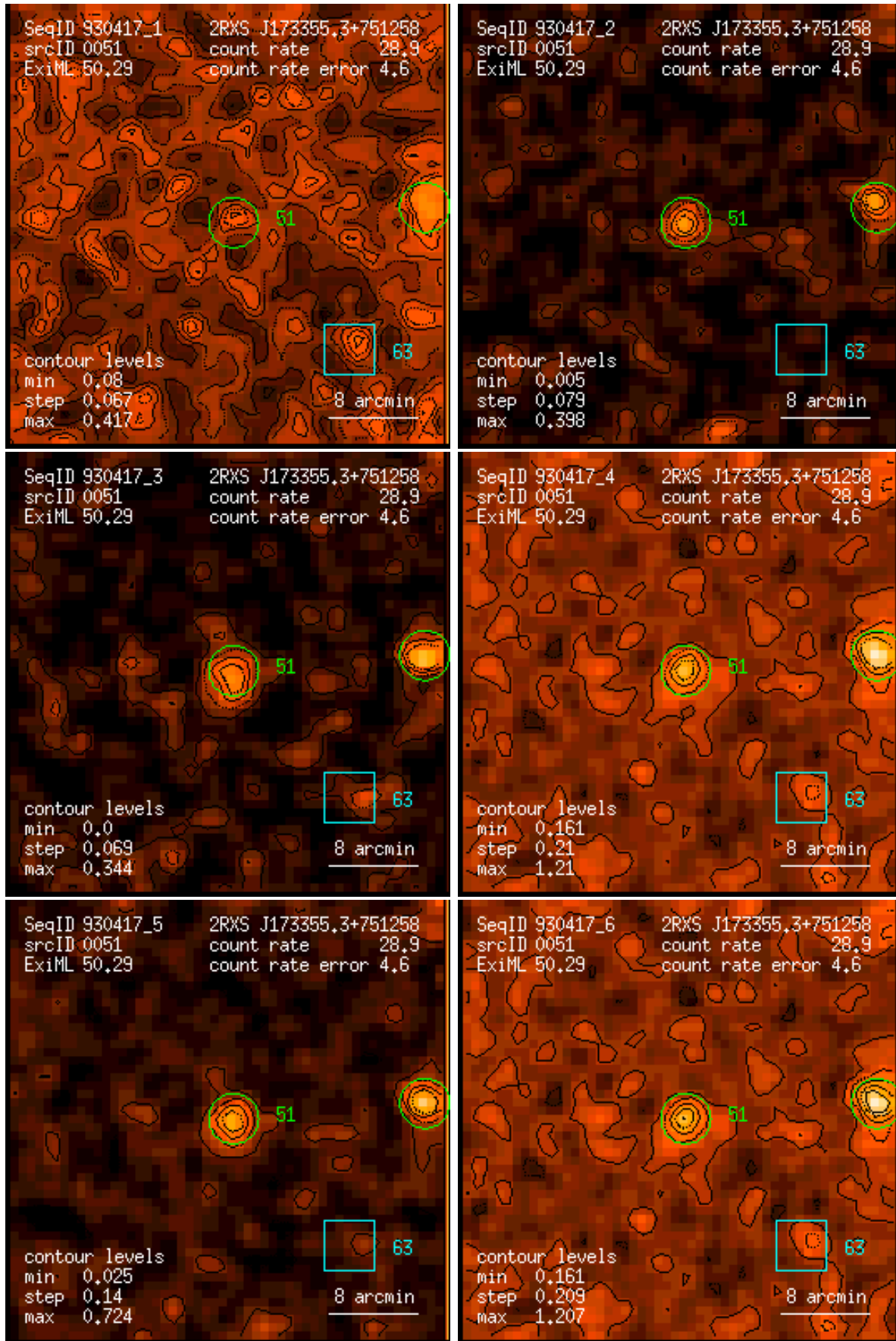
Figure 51: RASS 930417: detection 0051: band rate images, Gaussian filter: (1) PSPC channels 11 – 41, (2) 52 – 90, (3) 91 – 201, (4) 11 – 235, (5) 52 – 201, (6) 11 – 201. Broad band rates in counts/ks. Band rate contour levels in counts/ks/arcmin 2 .
