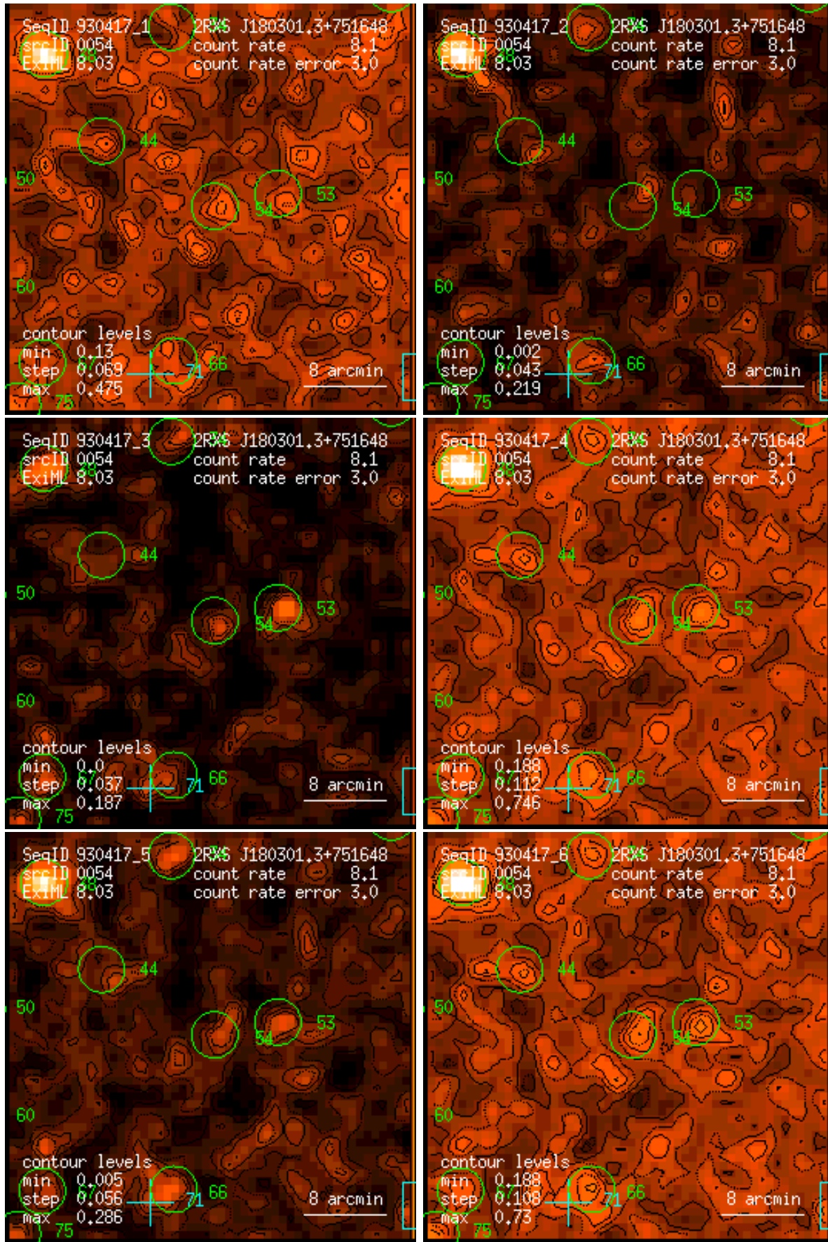
Figure 54: RASS 930417: detection 0054: band rate images, Gaussian filter: (1) PSPC channels 11 – 41, (2) 52 – 90, (3) 91 – 201, (4) 11 – 235, (5) 52 – 201, (6) 11 – 201. Broad band rates in counts/ks. Band rate contour levels in counts/ks/arcmin 2 .
