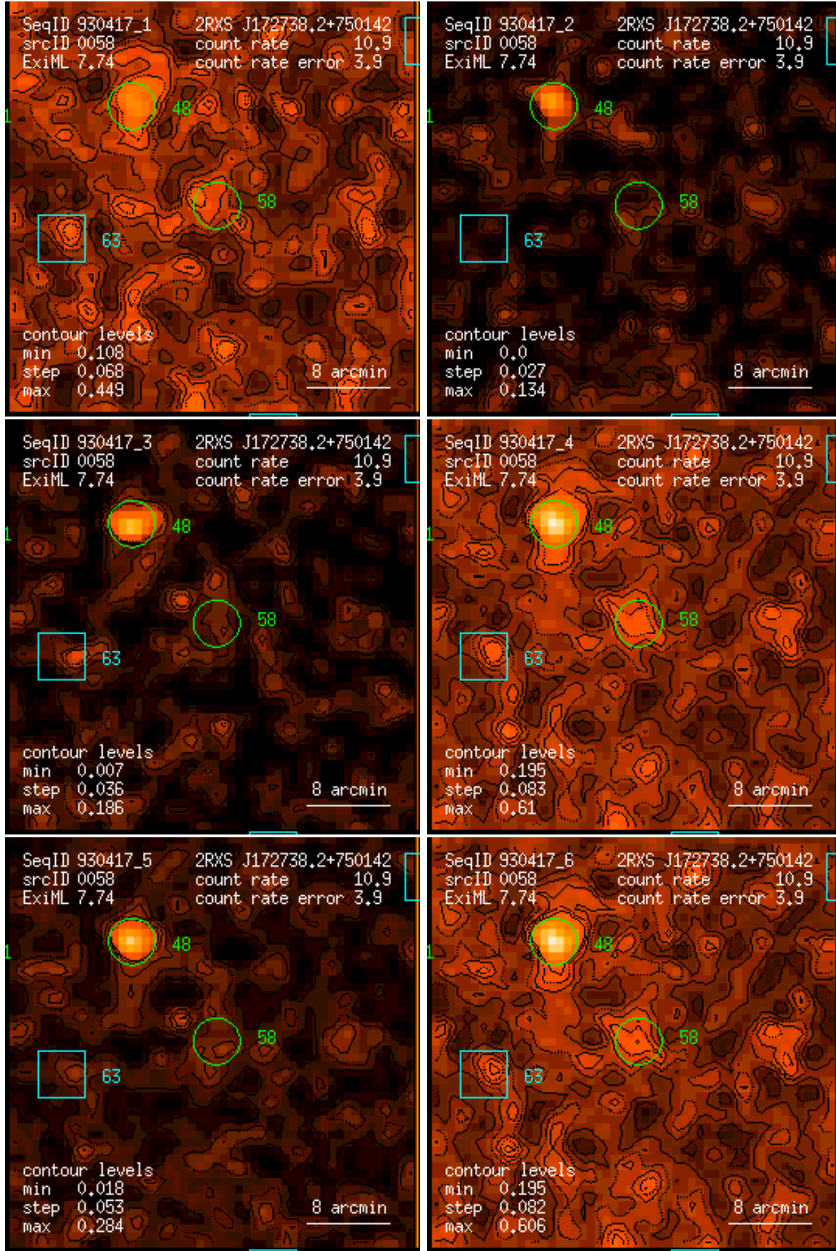
Figure 58: RASS 930417: detection 0058: band rate images, Gaussian filter: (1) PSPC channels 11 – 41, (2) 52 – 90, (3) 91 – 201, (4) 11 – 235, (5) 52 – 201, (6) 11 – 201. Broad band rates in counts/ks. Band rate contour levels in counts/ks/arcmin 2 .
