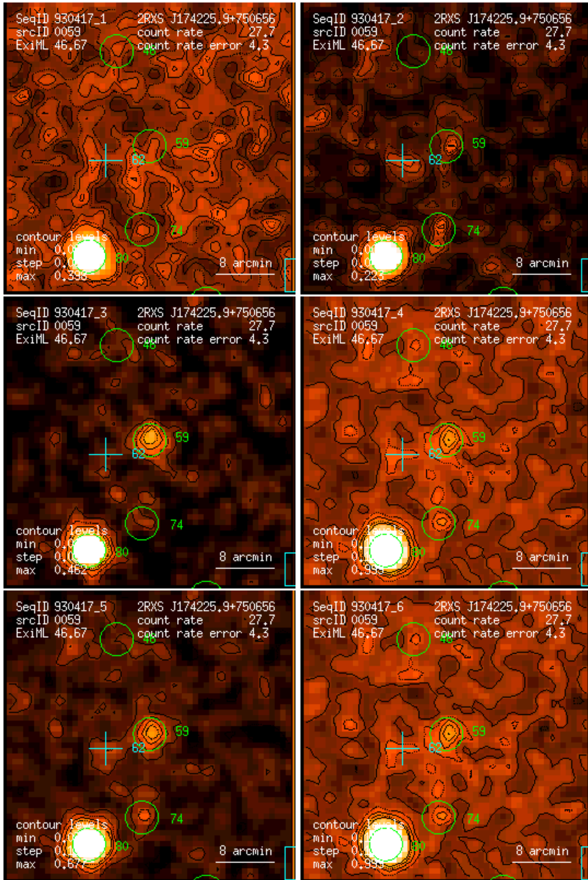
Figure 59: RASS 930417: detection 0059: band rate images, Gaussian filter: (1) PSPC channels 11 – 41, (2) 52 – 90, (3) 91 – 201, (4) 11 – 235, (5) 52 – 201, (6) 11 – 201. Broad band rates in counts/ks. Band rate contour levels in counts/ks/arcmin 2 .
