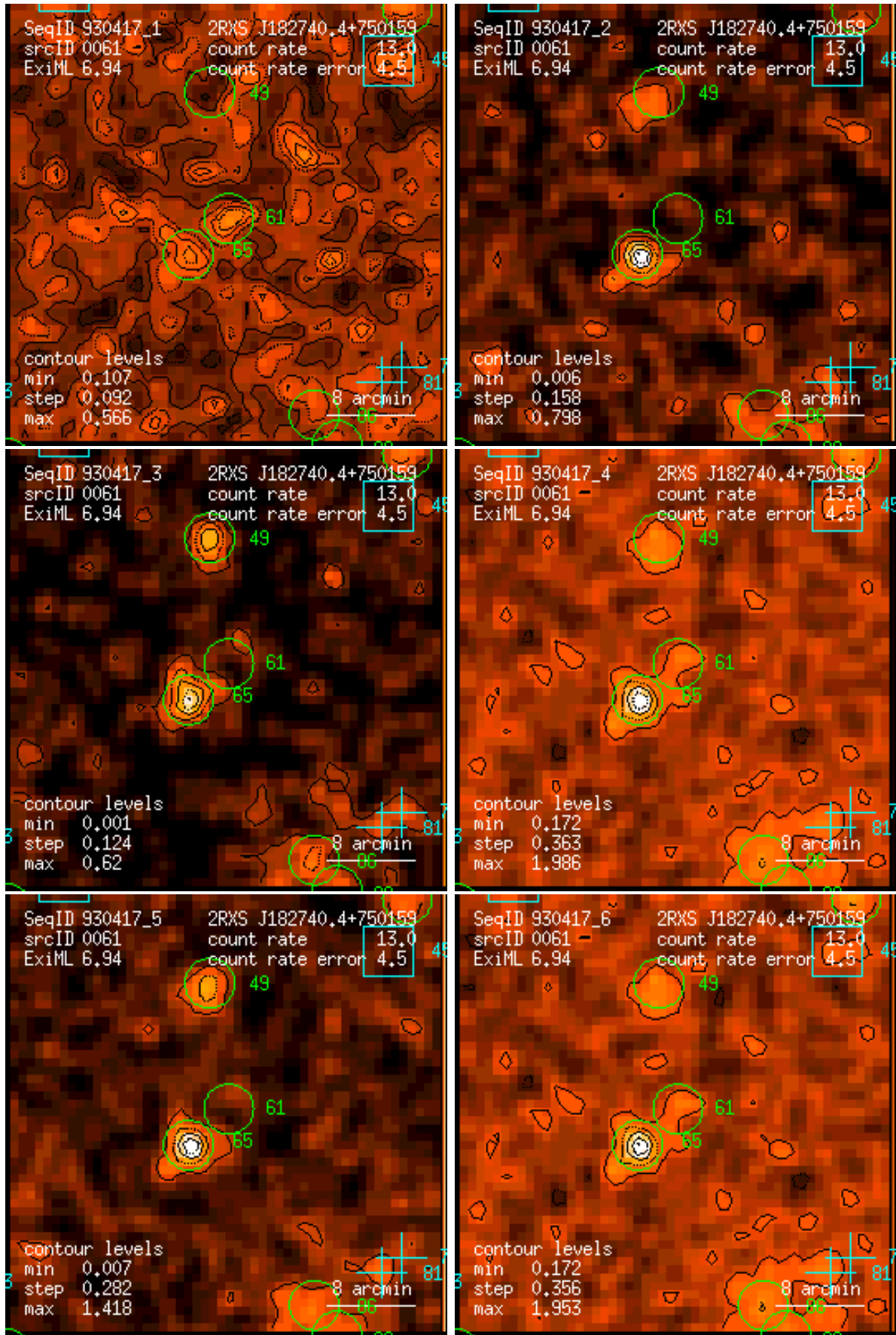
Figure 61: RASS 930417: detection 0061: band rate images, Gaussian filter: (1) PSPC channels 11 – 41, (2) 52 – 90, (3) 91 – 201, (4) 11 – 235, (5) 52 – 201, (6) 11 – 201. Broad band rates in counts/ks. Band rate contour levels in counts/ks/arcmin 2 .
