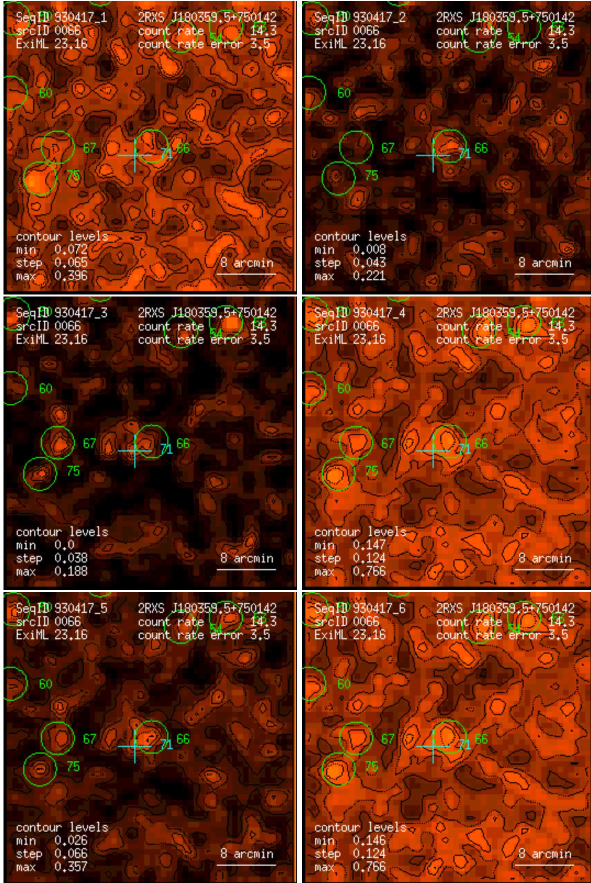
Figure 66: RASS 930417: detection 0066: band rate images, Gaussian filter: (1) PSPC channels 11 – 41, (2) 52 – 90, (3) 91 – 201, (4) 11 – 235, (5) 52 – 201, (6) 11 – 201. Broad band rates in counts/ks. Band rate contour levels in counts/ks/arcmin 2 .
