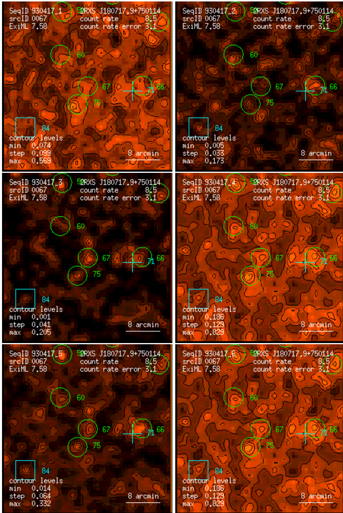
Figure 67: RASS 930417: detection 0067: band rate images, Gaussian filter: (1) PSPC channels 11 – 41, (2) 52 – 90, (3) 91 – 201, (4) 11 – 235, (5) 52 – 201, (6) 11 – 201. Broad band rates in counts/ks. Band rate contour levels in counts/ks/arcmin 2 .
