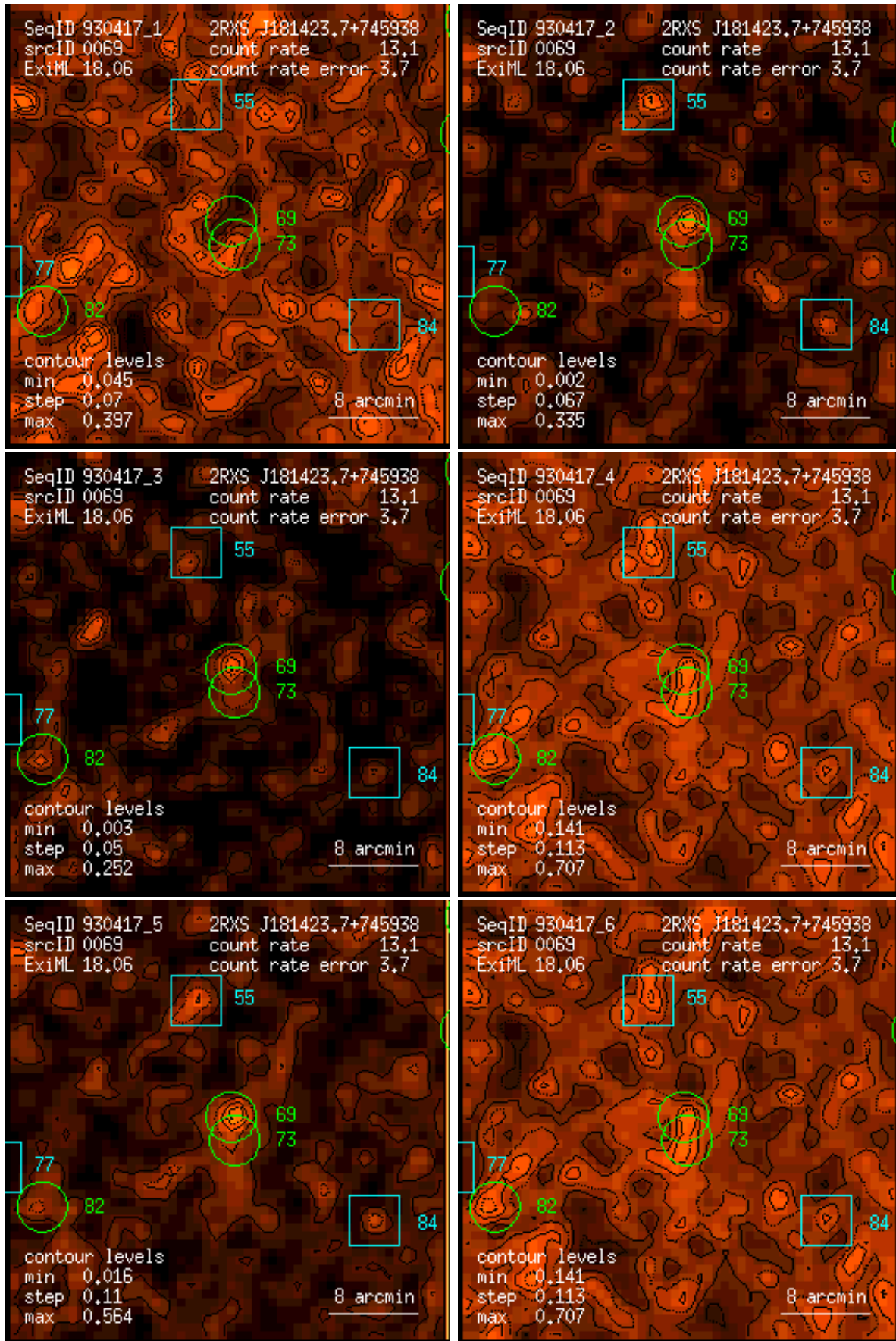
Figure 69: RASS 930417: detection 0069: band rate images, Gaussian filter: (1) PSPC channels 11 – 41, (2) 52 – 90, (3) 91 – 201, (4) 11 – 235, (5) 52 – 201, (6) 11 – 201. Broad band rates in counts/ks. Band rate contour levels in counts/ks/arcmin 2 .
