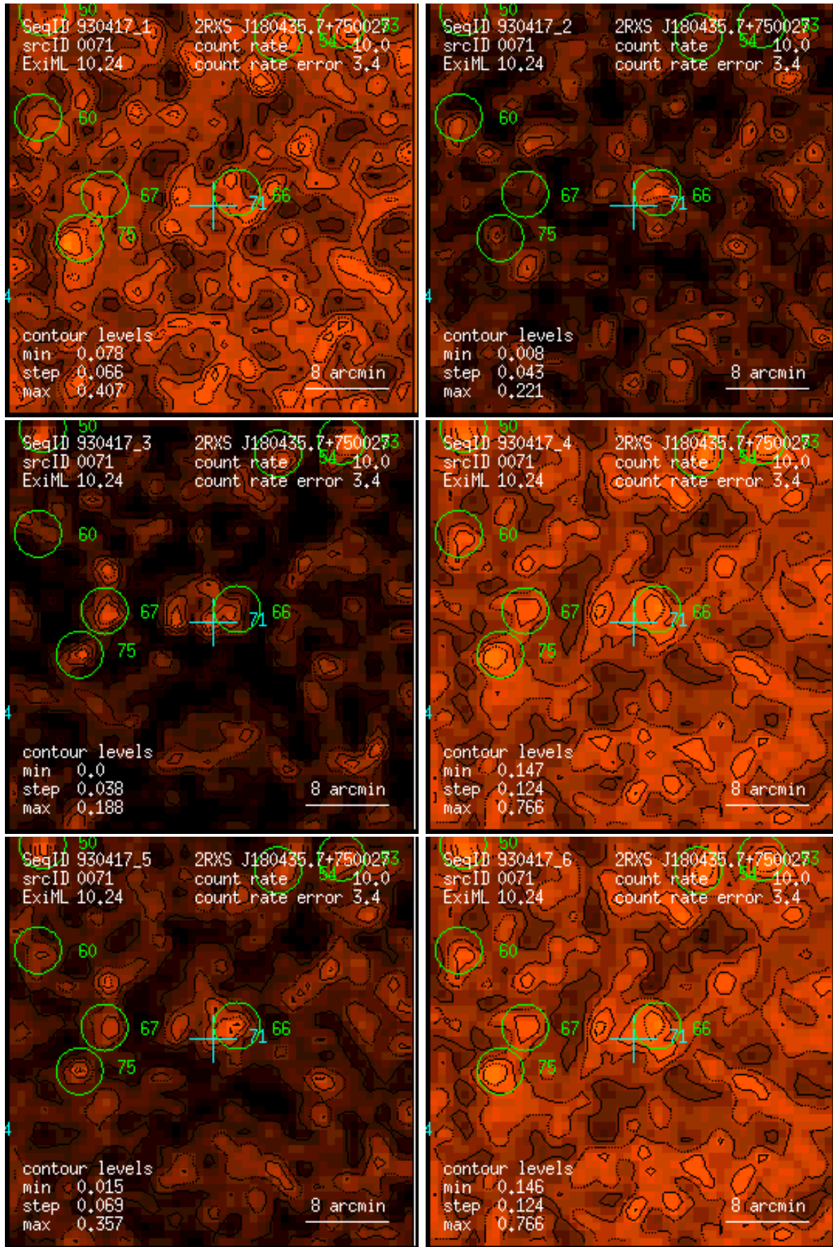
Figure 71: RASS 930417: detection 0071: band rate images, Gaussian filter: (1) PSPC channels 11 – 41, (2) 52 – 90, (3) 91 – 201, (4) 11 – 235, (5) 52 – 201, (6) 11 – 201. Broad band rates in counts/ks. Band rate contour levels in counts/ks/arcmin 2 .
