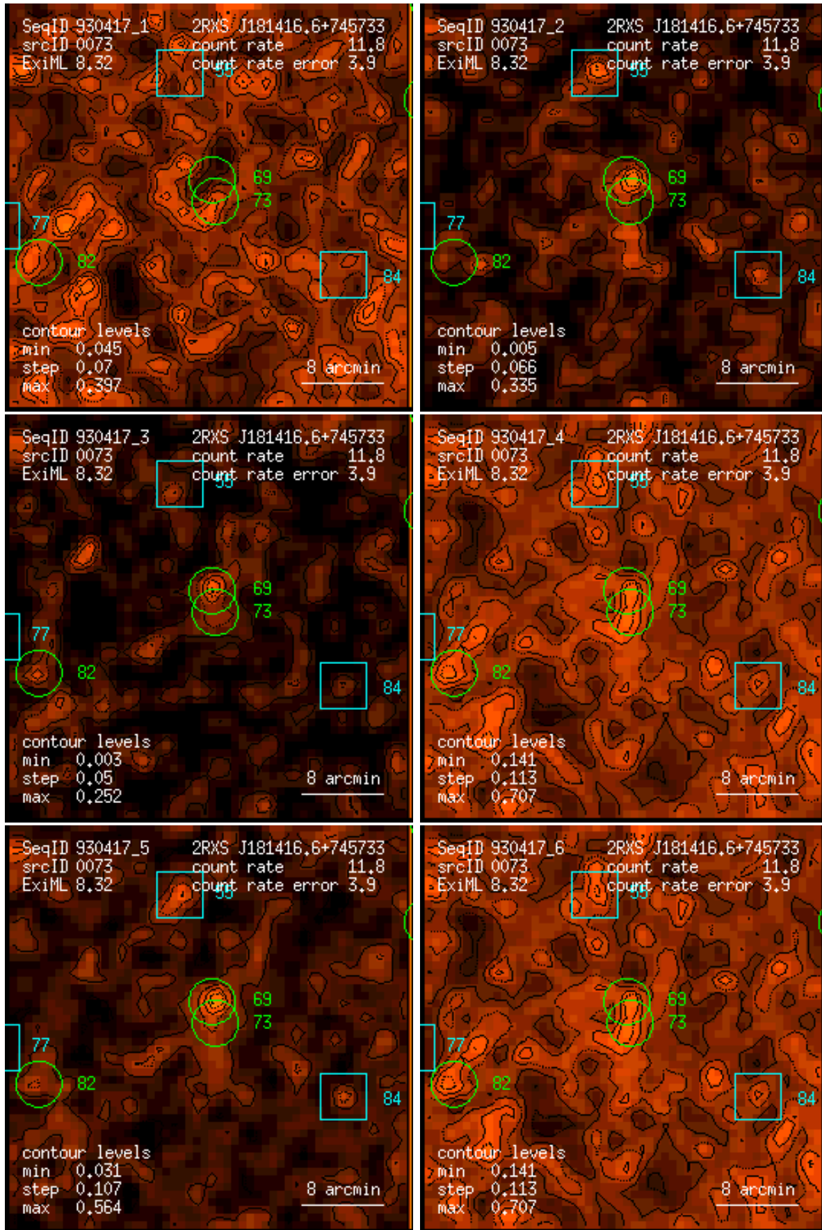
Figure 73: RASS 930417: detection 0073: band rate images, Gaussian filter: (1) PSPC channels 11 – 41, (2) 52 – 90, (3) 91 – 201, (4) 11 – 235, (5) 52 – 201, (6) 11 – 201. Broad band rates in counts/ks. Band rate contour levels in counts/ks/arcmin 2 .
