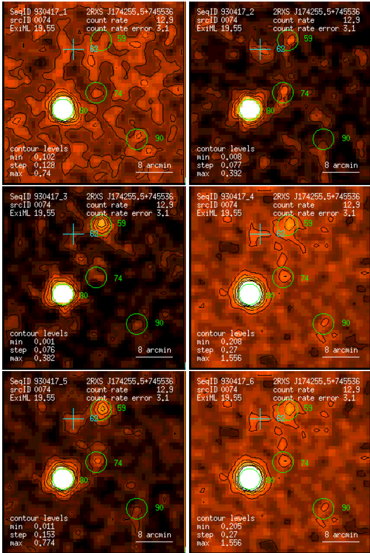
Figure 74: RASS 930417: detection 0074: band rate images, Gaussian filter: (1) PSPC channels 11 – 41, (2) 52 – 90, (3) 91 – 201, (4) 11 – 235, (5) 52 – 201, (6) 11 – 201. Broad band rates in counts/ks. Band rate contour levels in counts/ks/arcmin 2 .
