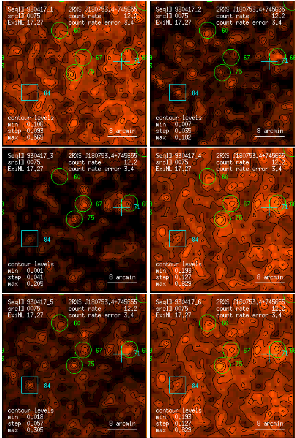
Figure 75: RASS 930417: detection 0075: band rate images, Gaussian filter: (1) PSPC channels 11 – 41, (2) 52 – 90, (3) 91 – 201, (4) 11 – 235, (5) 52 – 201, (6) 11 – 201. Broad band rates in counts/ks. Band rate contour levels in counts/ks/arcmin 2 .
