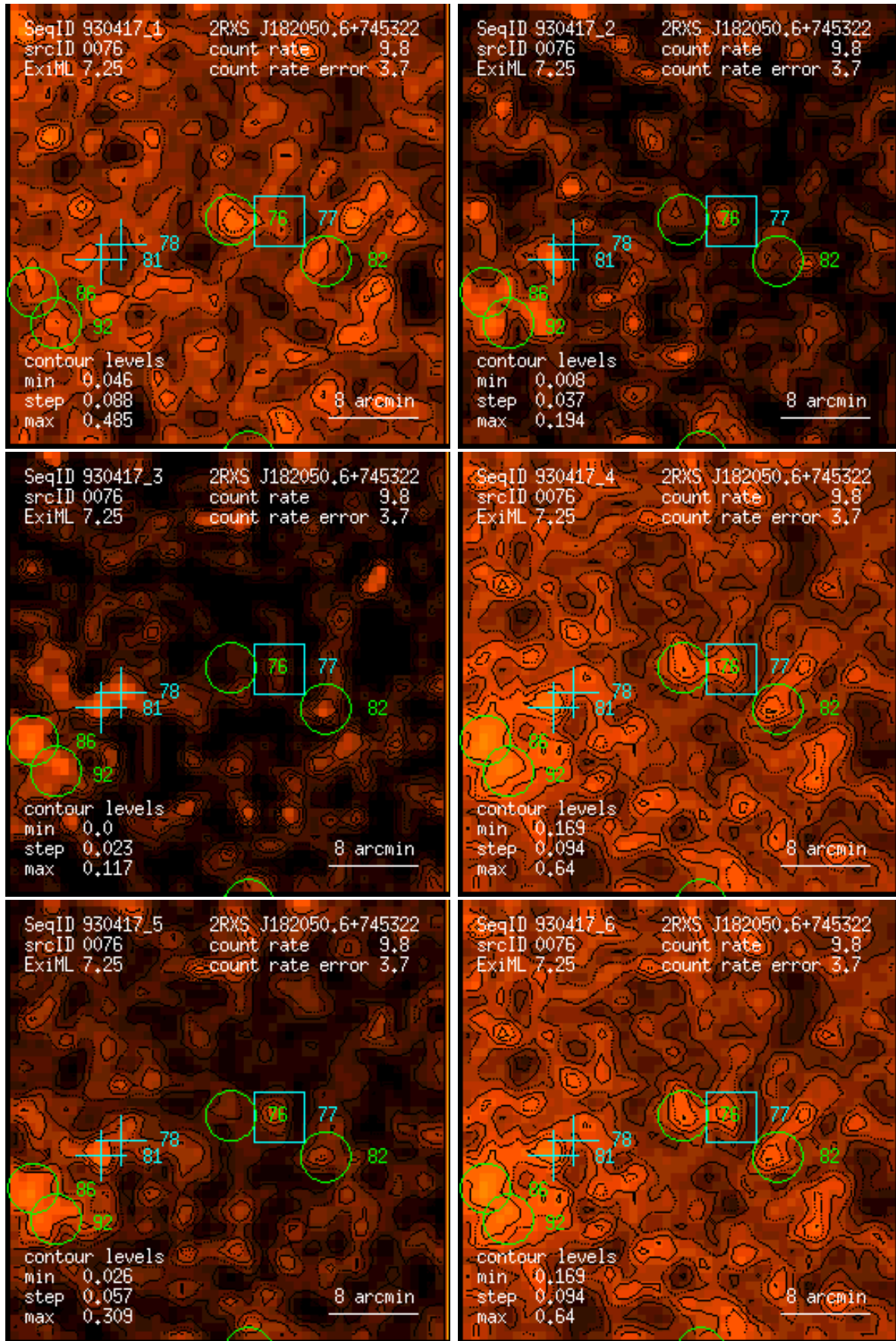
Figure 76: RASS 930417: detection 0076: band rate images, Gaussian filter: (1) PSPC channels 11 – 41, (2) 52 – 90, (3) 91 – 201, (4) 11 – 235, (5) 52 – 201, (6) 11 – 201. Broad band rates in counts/ks. Band rate contour levels in counts/ks/arcmin 2 .
