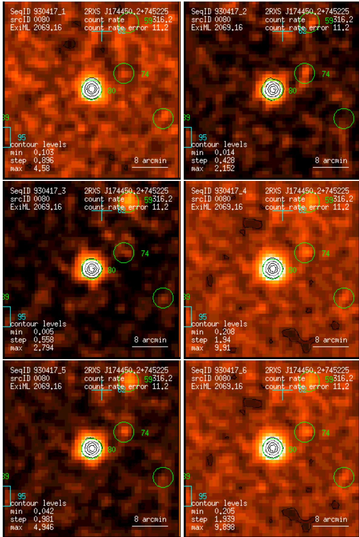
Figure 80: RASS 930417: detection 0080: band rate images, Gaussian filter: (1) PSPC channels 11 – 41, (2) 52 – 90, (3) 91 – 201, (4) 11 – 235, (5) 52 – 201, (6) 11 – 201. Broad band rates in counts/ks. Band rate contour levels in counts/ks/arcmin 2 .
