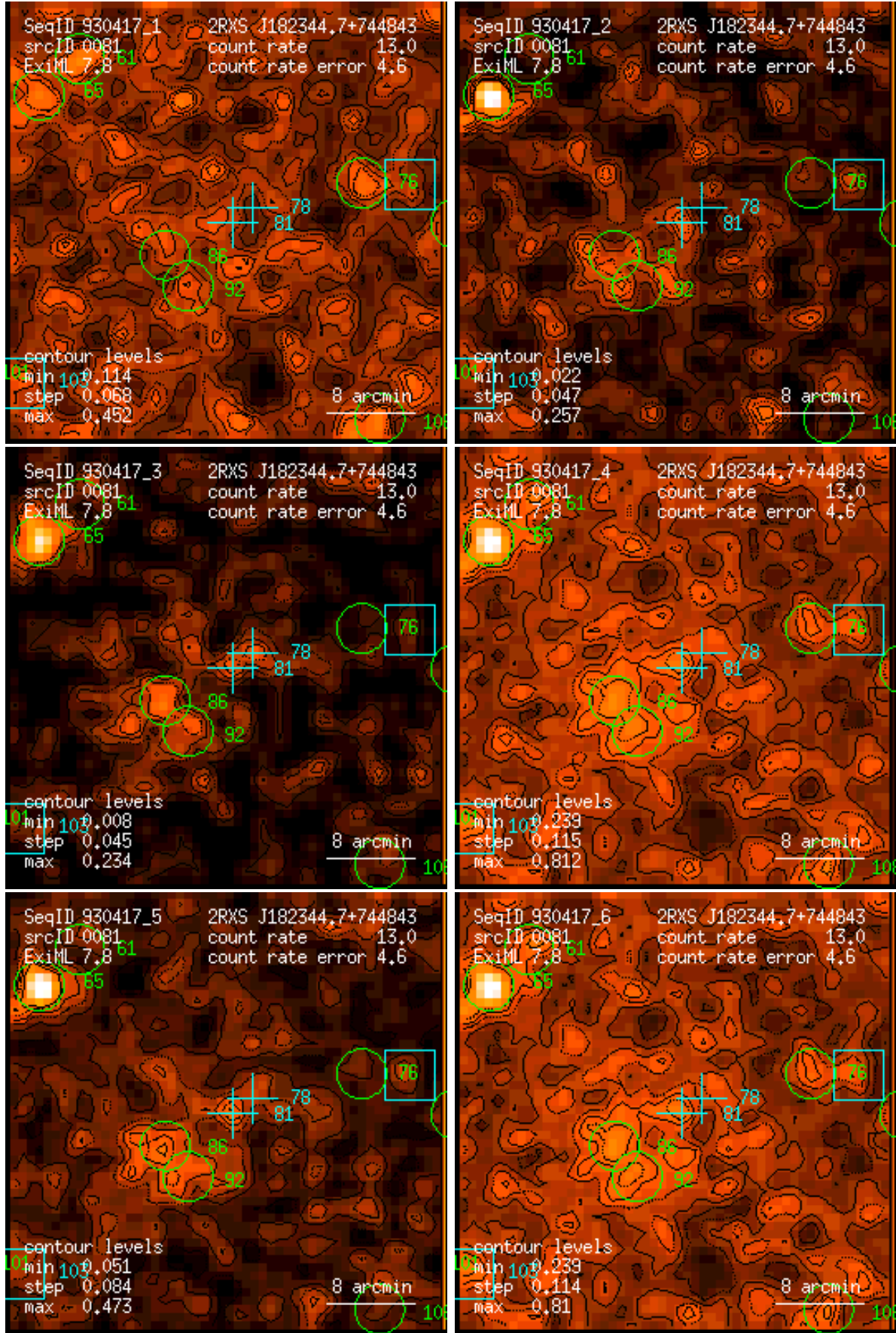
Figure 81: RASS 930417: detection 0081: band rate images, Gaussian filter: (1) PSPC channels 11 – 41, (2) 52 – 90, (3) 91 – 201, (4) 11 – 235, (5) 52 – 201, (6) 11 – 201. Broad band rates in counts/ks. Band rate contour levels in counts/ks/arcmin 2 .
