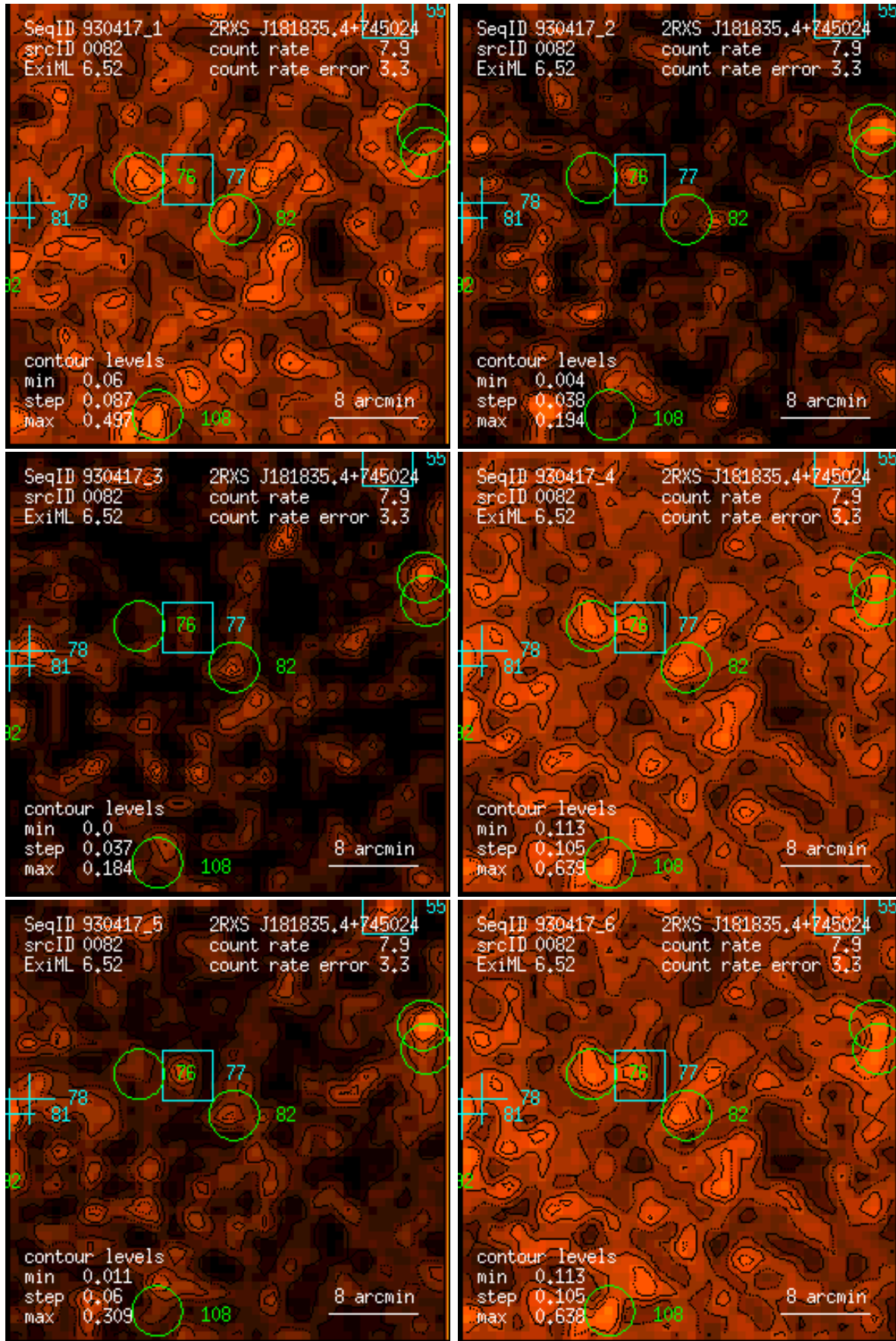
Figure 82: RASS 930417: detection 0082: band rate images, Gaussian filter: (1) PSPC channels 11 – 41, (2) 52 – 90, (3) 91 – 201, (4) 11 – 235, (5) 52 – 201, (6) 11 – 201. Broad band rates in counts/ks. Band rate contour levels in counts/ks/arcmin 2 .
