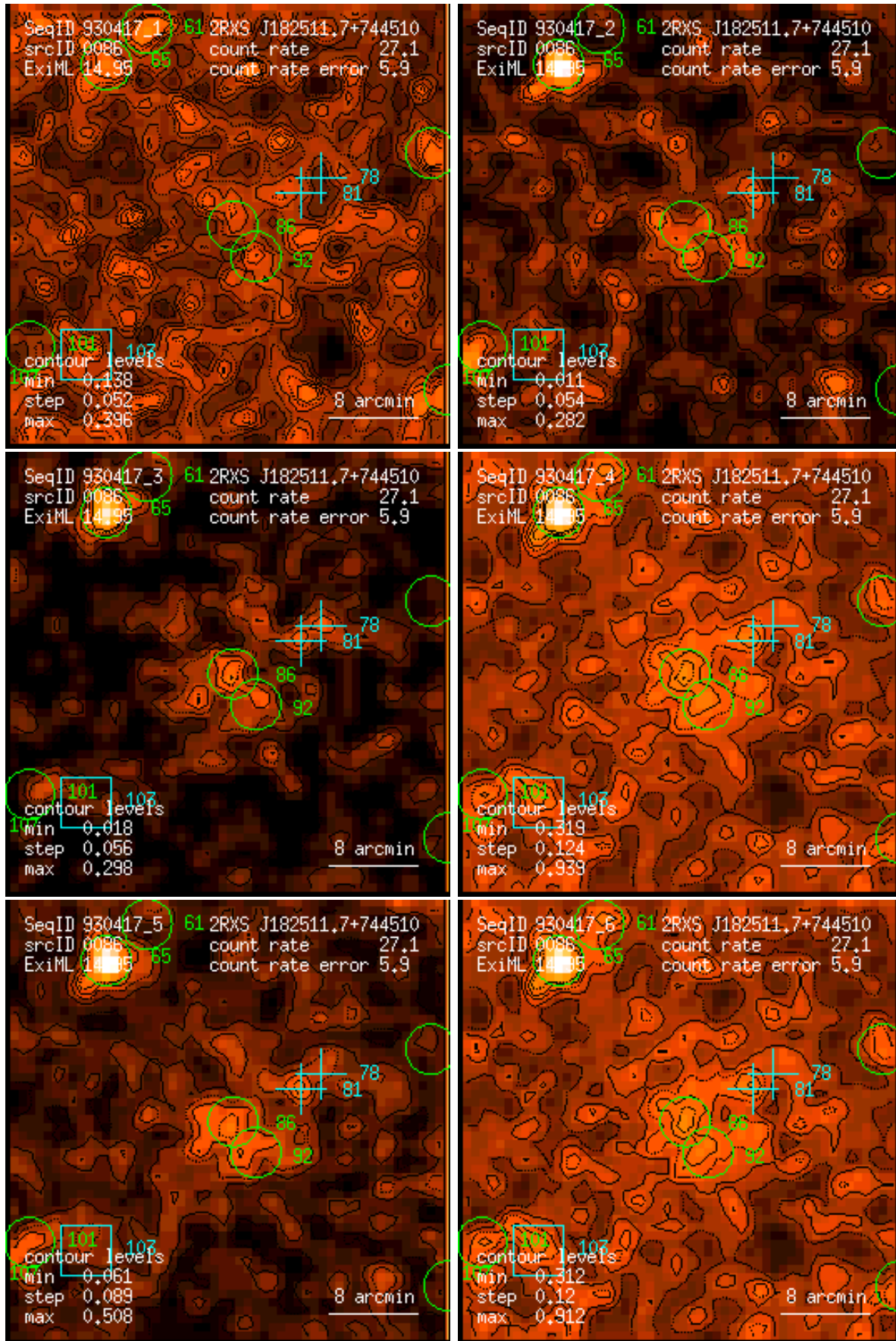
Figure 86: RASS 930417: detection 0086: band rate images, Gaussian filter: (1) PSPC channels 11 – 41, (2) 52 – 90, (3) 91 – 201, (4) 11 – 235, (5) 52 – 201, (6) 11 – 201. Broad band rates in counts/ks. Band rate contour levels in counts/ks/arcmin 2 .
