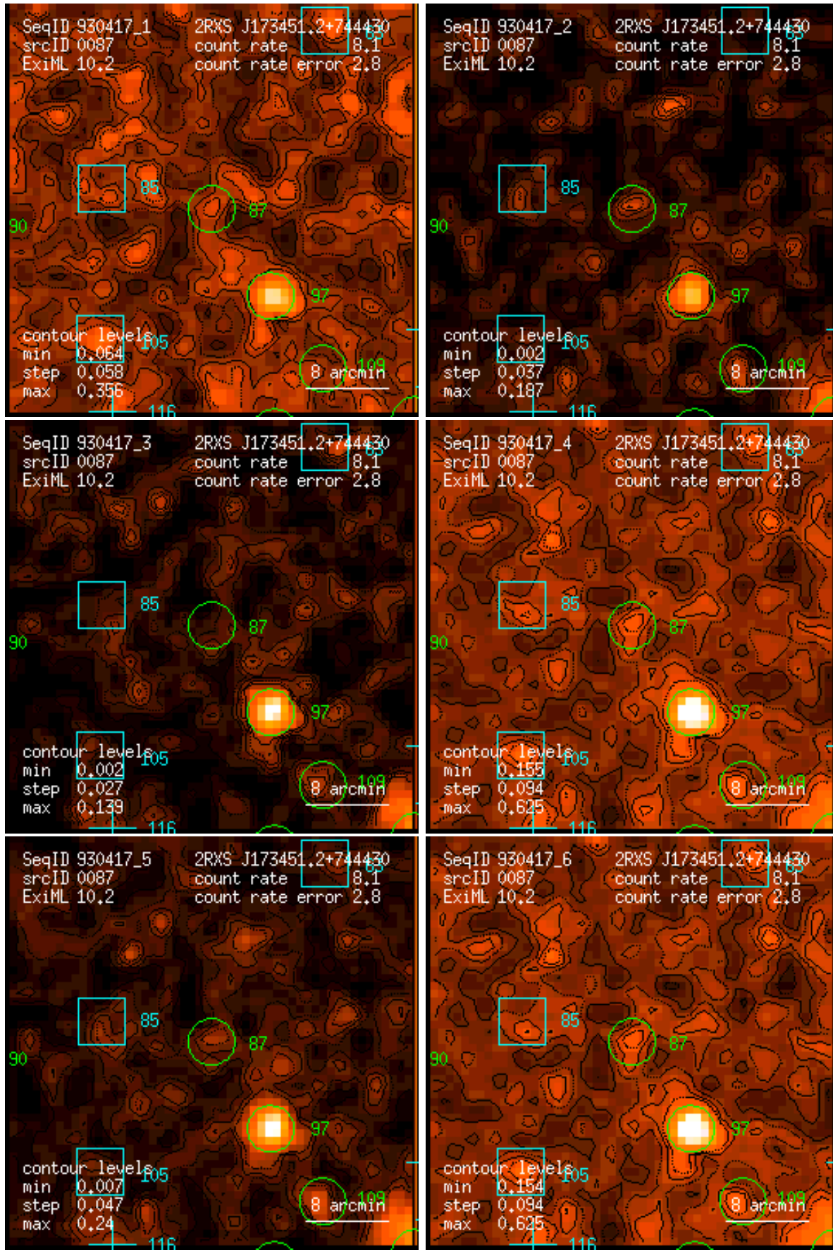
Figure 87: RASS 930417: detection 0087: band rate images, Gaussian filter: (1) PSPC channels 11 – 41, (2) 52 – 90, (3) 91 – 201, (4) 11 – 235, (5) 52 – 201, (6) 11 – 201. Broad band rates in counts/ks. Band rate contour levels in counts/ks/arcmin 2 .
