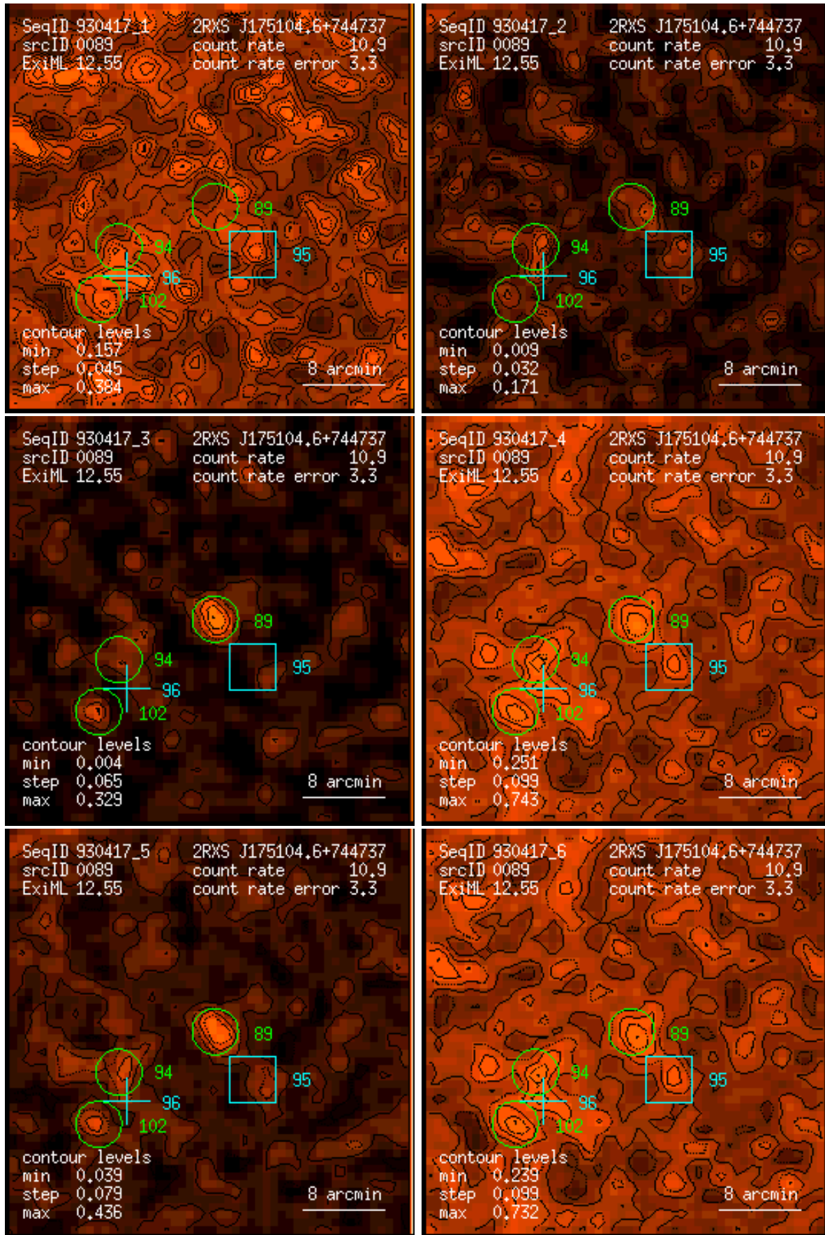
Figure 89: RASS 930417: detection 0089: band rate images, Gaussian filter: (1) PSPC channels 11 – 41, (2) 52 – 90, (3) 91 – 201, (4) 11 – 235, (5) 52 – 201, (6) 11 – 201. Broad band rates in counts/ks. Band rate contour levels in counts/ks/arcmin 2 .
