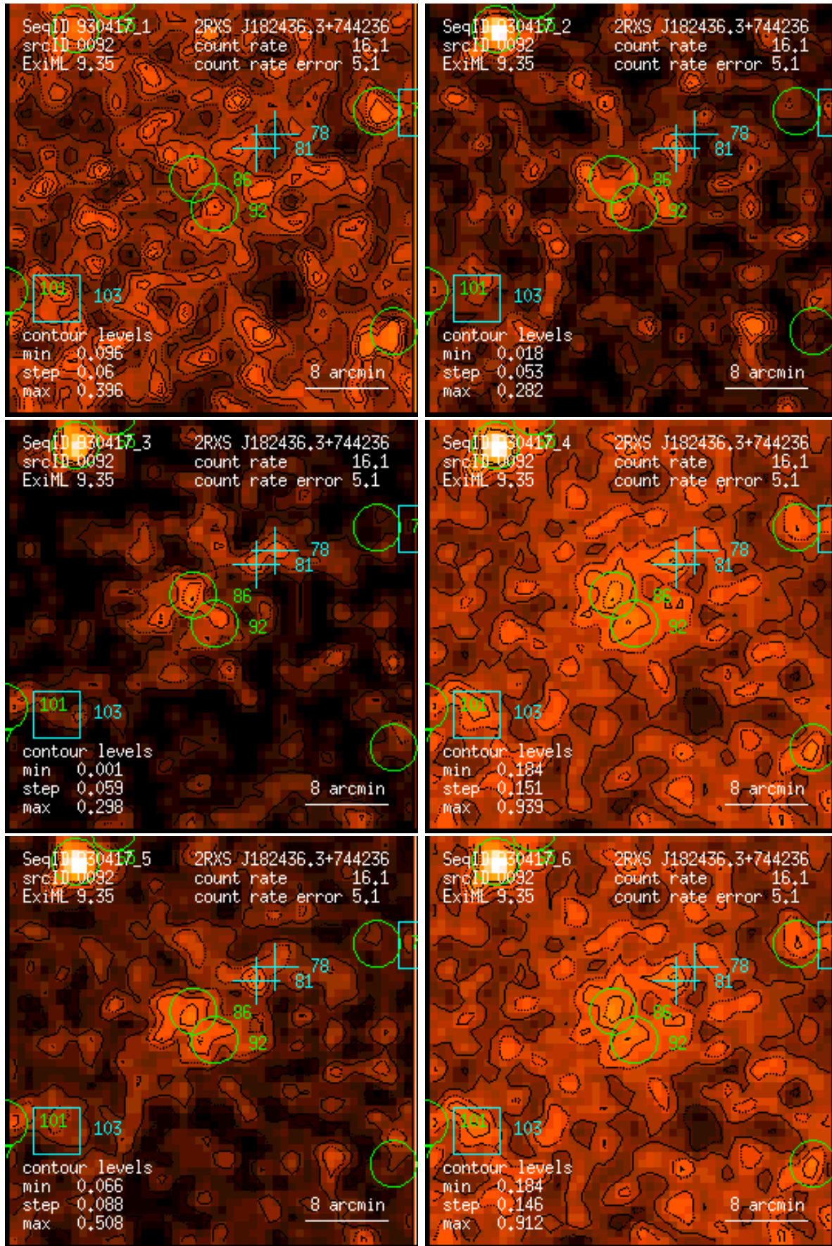
Figure 92: RASS 930417: detection 0092: band rate images, Gaussian filter: (1) PSPC channels 11 – 41, (2) 52 – 90, (3) 91 – 201, (4) 11 – 235, (5) 52 – 201, (6) 11 – 201. Broad band rates in counts/ks. Band rate contour levels in counts/ks/arcmin 2 .
