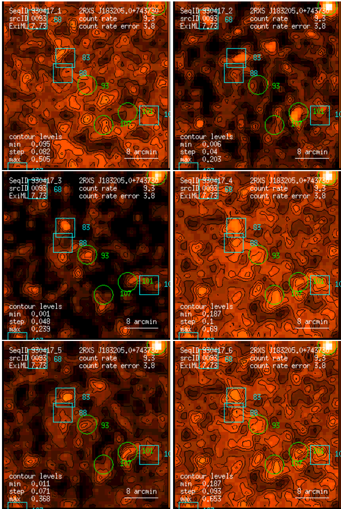
Figure 93: RASS 930417: detection 0093: band rate images, Gaussian filter: (1) PSPC channels 11 – 41, (2) 52 – 90, (3) 91 – 201, (4) 11 – 235, (5) 52 – 201, (6) 11 – 201. Broad band rates in counts/ks. Band rate contour levels in counts/ks/arcmin 2 .
