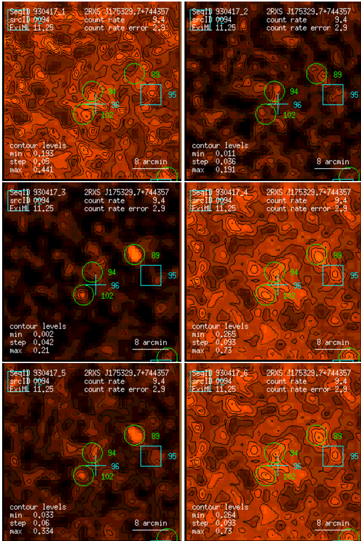
Figure 94: RASS 930417: detection 0094: band rate images, Gaussian filter: (1) PSPC channels 11 – 41, (2) 52 – 90, (3) 91 – 201, (4) 11 – 235, (5) 52 – 201, (6) 11 – 201. Broad band rates in counts/ks. Band rate contour levels in counts/ks/arcmin 2 .
