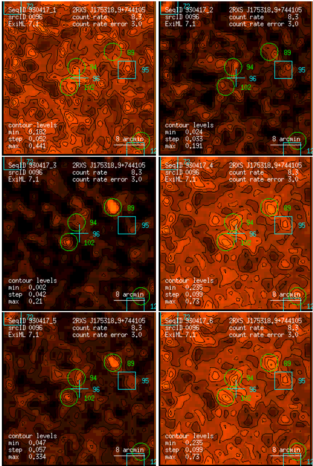
Figure 96: RASS 930417: detection 0096: band rate images, Gaussian filter: (1) PSPC channels 11 – 41, (2) 52 – 90, (3) 91 – 201, (4) 11 – 235, (5) 52 – 201, (6) 11 – 201. Broad band rates in counts/ks. Band rate contour levels in counts/ks/arcmin 2 .
