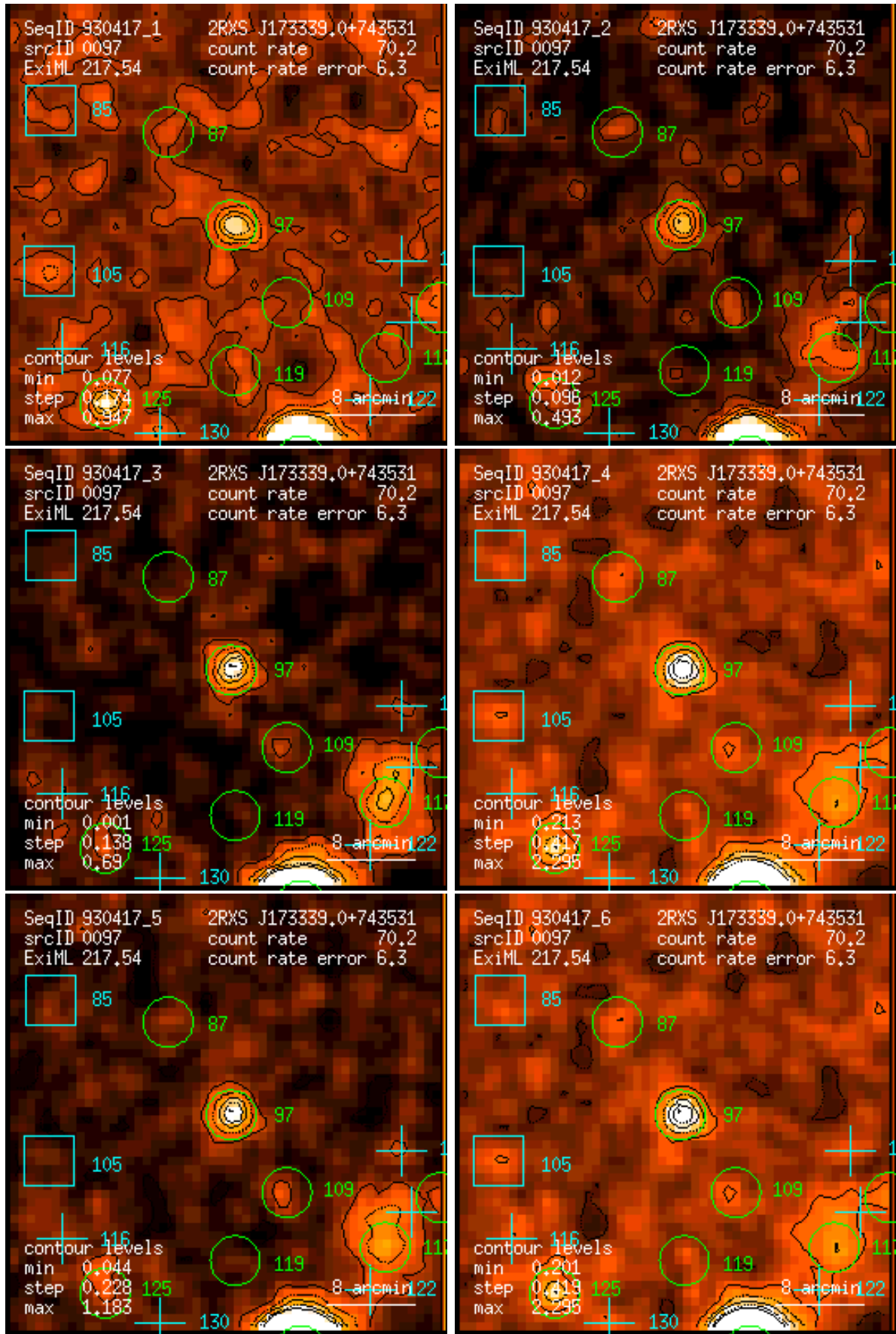
Figure 97: RASS 930417: detection 0097: band rate images, Gaussian filter: (1) PSPC channels 11 – 41, (2) 52 – 90, (3) 91 – 201, (4) 11 – 235, (5) 52 – 201, (6) 11 – 201. Broad band rates in counts/ks. Band rate contour levels in counts/ks/arcmin 2 .
