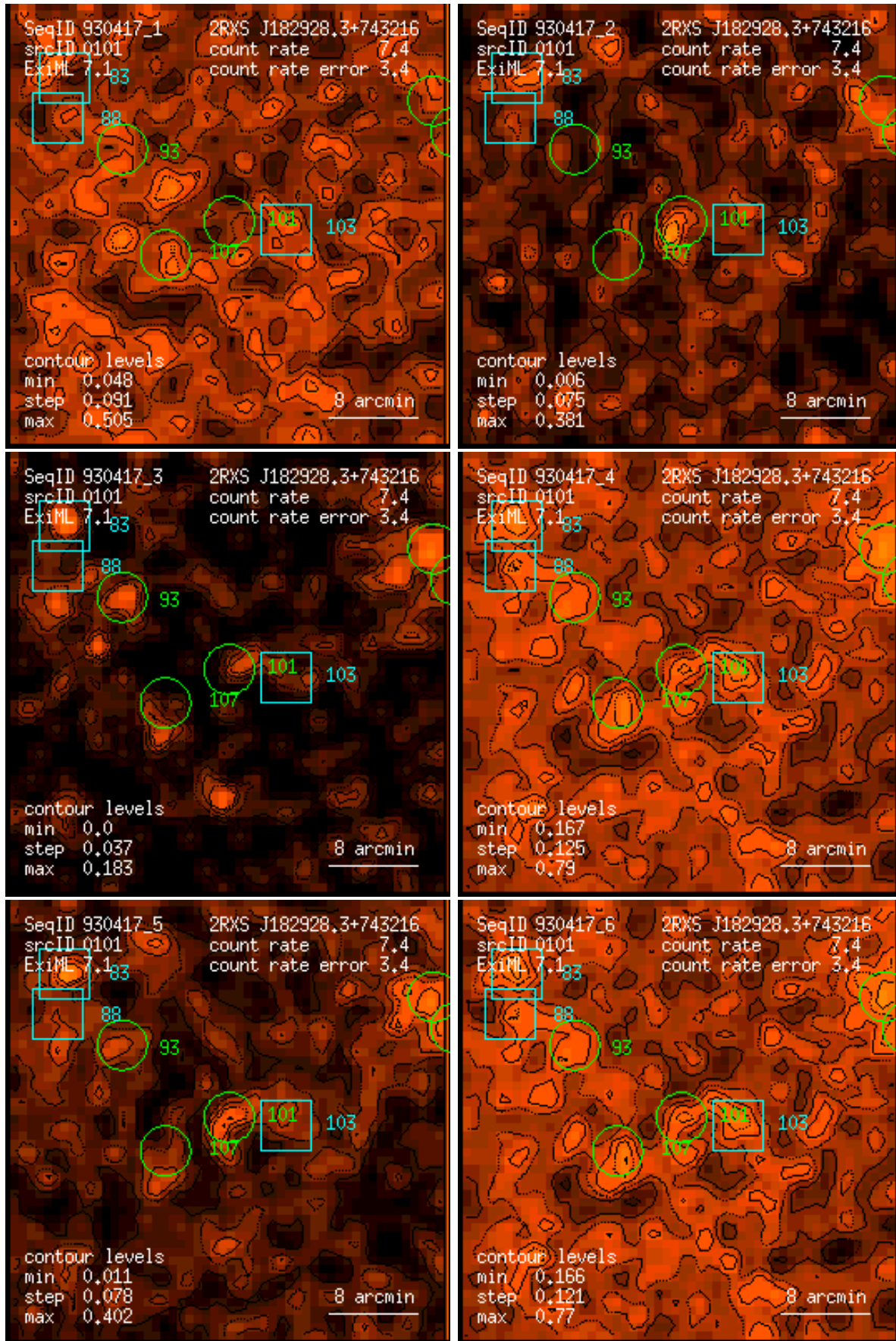
Figure 101: RASS 930417: detection 0101: band rate images, Gaussian filter: (1) PSPC channels 11 – 41, (2) 52 – 90, (3) 91 – 201, (4) 11 – 235, (5) 52 – 201, (6) 11 – 201. Broad band rates in counts/ks. Band rate contour levels in counts/ks/arcmin 2 .
