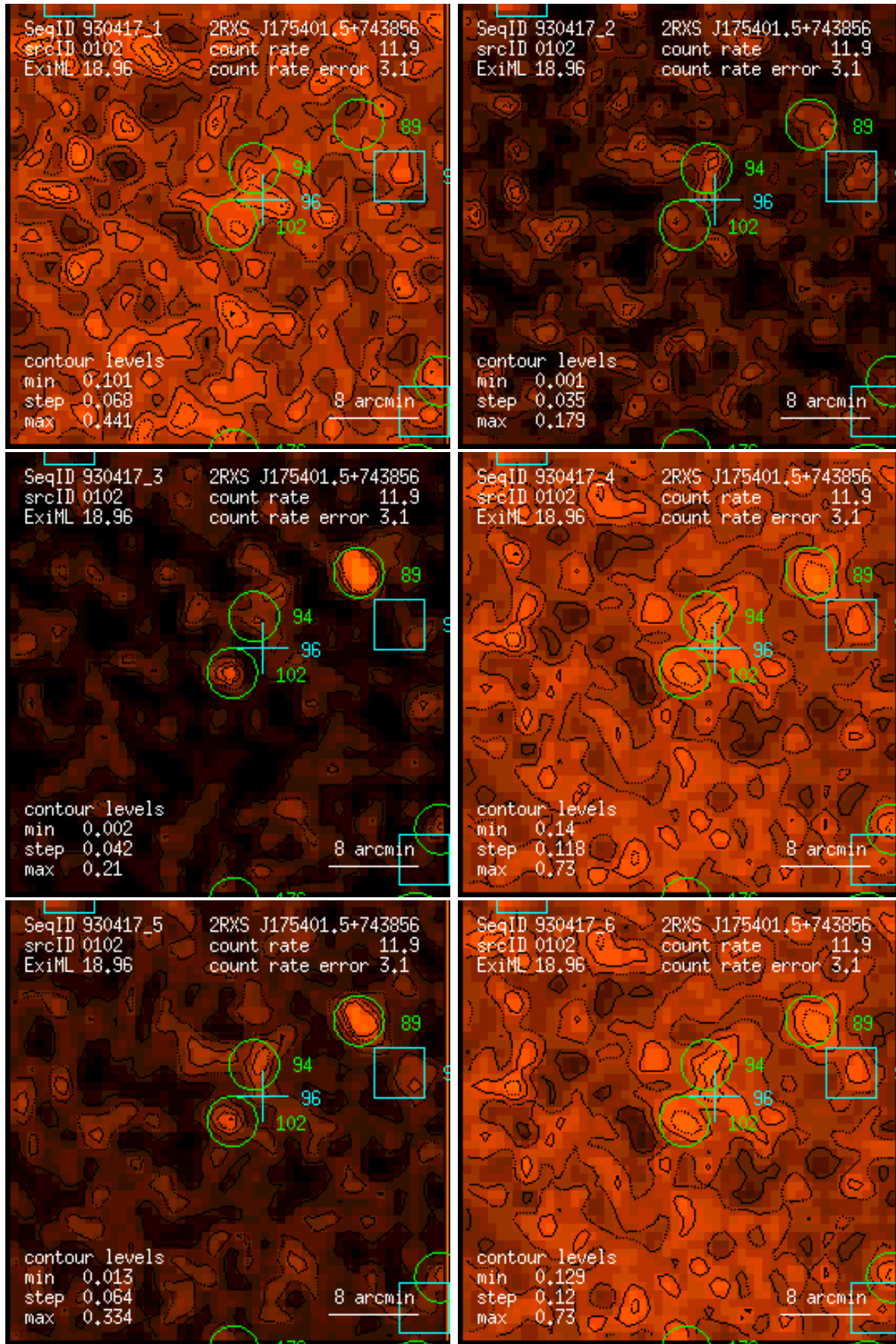
Figure 102: RASS 930417: detection 0102: band rate images, Gaussian filter: (1) PSPC channels 11 – 41, (2) 52 – 90, (3) 91 – 201, (4) 11 – 235, (5) 52 – 201, (6) 11 – 201. Broad band rates in counts/ks. Band rate contour levels in counts/ks/arcmin 2 .
