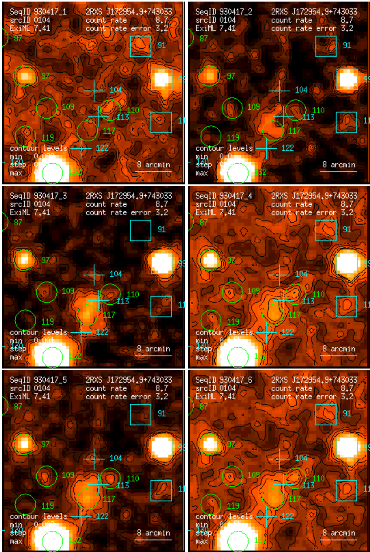
Figure 104: RASS 930417: detection 0104: band rate images, Gaussian filter: (1) PSPC channels 11 – 41, (2) 52 – 90, (3) 91 – 201, (4) 11 – 235, (5) 52 – 201, (6) 11 – 201. Broad band rates in counts/ks. Band rate contour levels in counts/ks/arcmin 2 .
