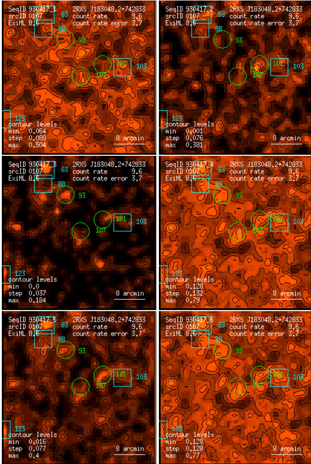
Figure 107: RASS 930417: detection 0107: band rate images, Gaussian filter: (1) PSPC channels 11 – 41, (2) 52 – 90, (3) 91 – 201, (4) 11 – 235, (5) 52 – 201, (6) 11 – 201. Broad band rates in counts/ks. Band rate contour levels in counts/ks/arcmin 2 .
