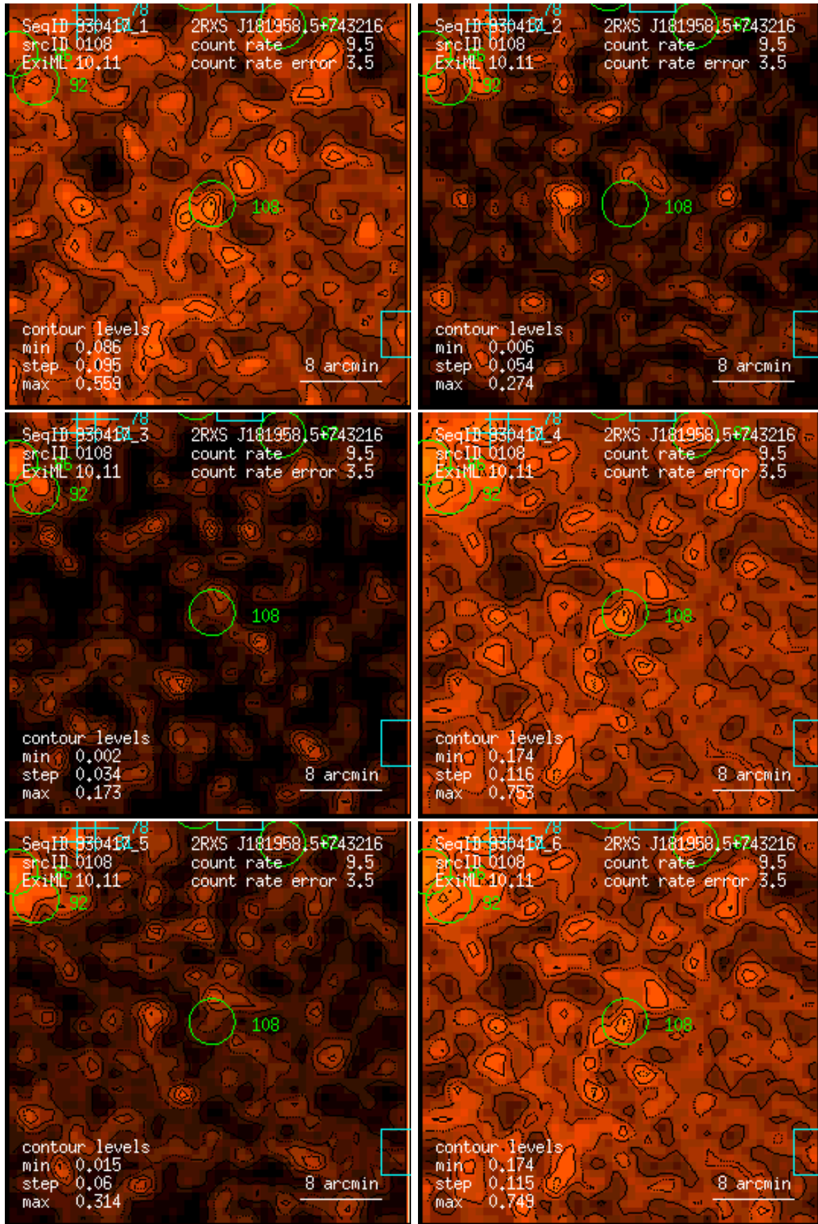
Figure 108: RASS 930417: detection 0108: band rate images, Gaussian filter: (1) PSPC channels 11 – 41, (2) 52 – 90, (3) 91 – 201, (4) 11 – 235, (5) 52 – 201, (6) 11 – 201. Broad band rates in counts/ks. Band rate contour levels in counts/ks/arcmin 2 .
