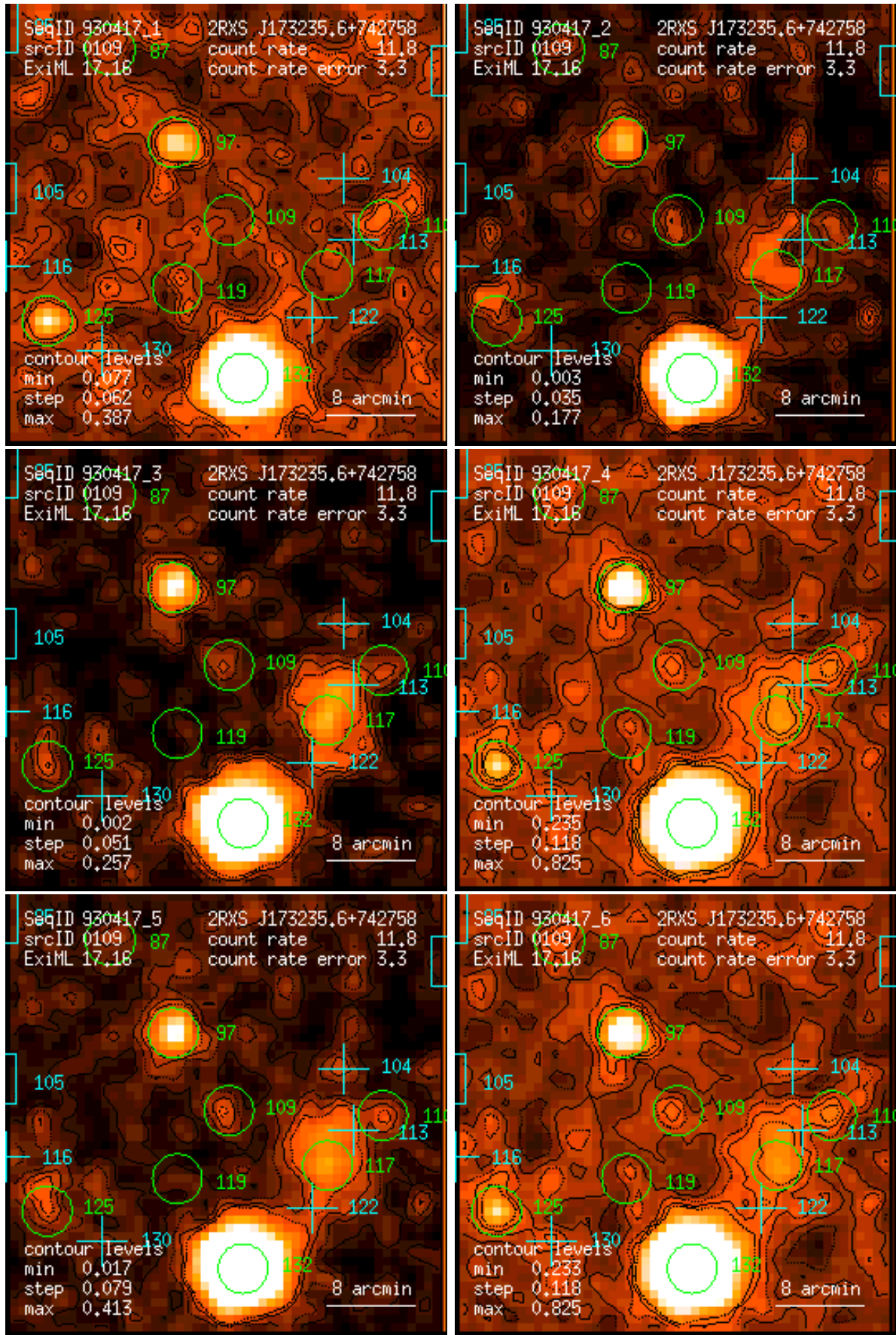
Figure 109: RASS 930417: detection 0109: band rate images, Gaussian filter: (1) PSPC channels 11 – 41, (2) 52 – 90, (3) 91 – 201, (4) 11 – 235, (5) 52 – 201, (6) 11 – 201. Broad band rates in counts/ks. Band rate contour levels in counts/ks/arcmin 2 .
