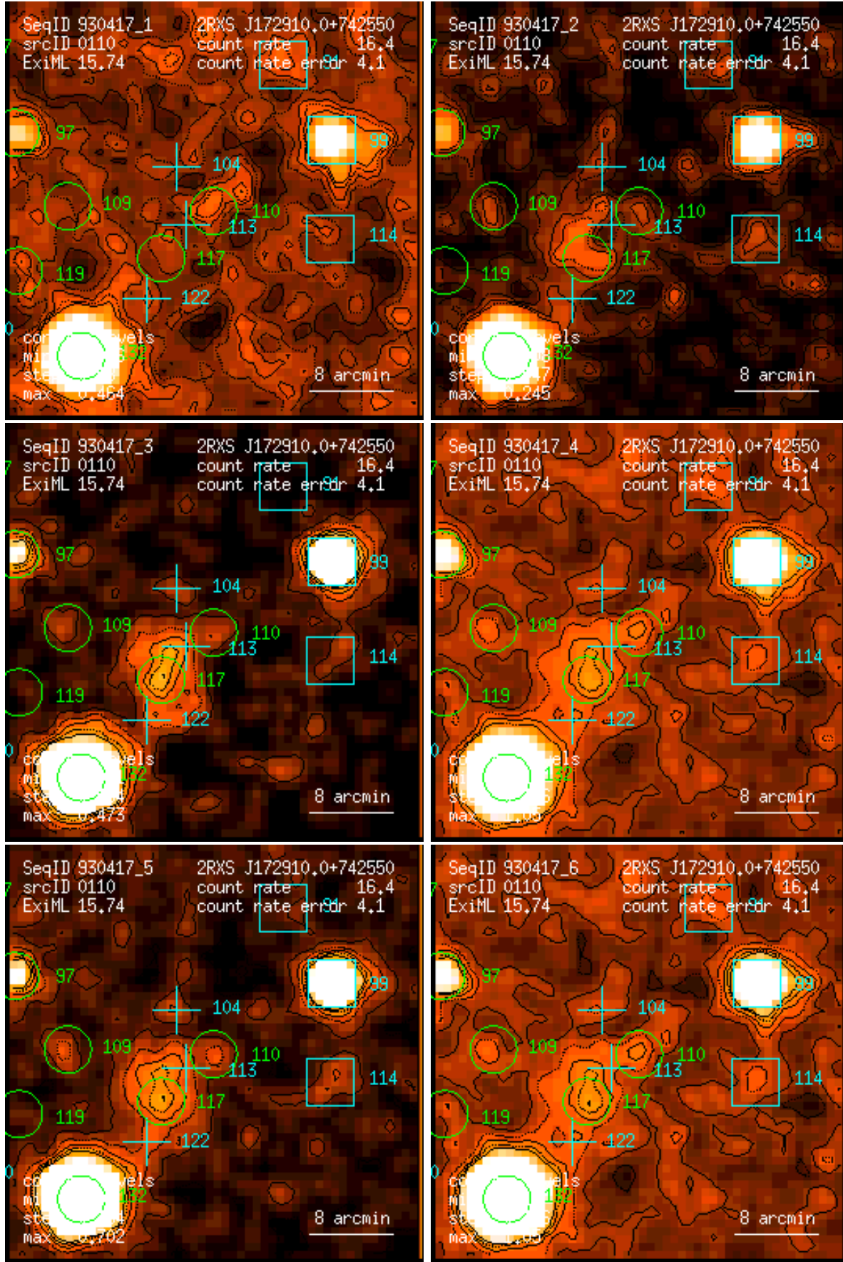
Figure 110: RASS 930417: detection 0110: band rate images, Gaussian filter: (1) PSPC channels 11 – 41, (2) 52 – 90, (3) 91 – 201, (4) 11 – 235, (5) 52 – 201, (6) 11 – 201. Broad band rates in counts/ks. Band rate contour levels in counts/ks/arcmin 2 .
