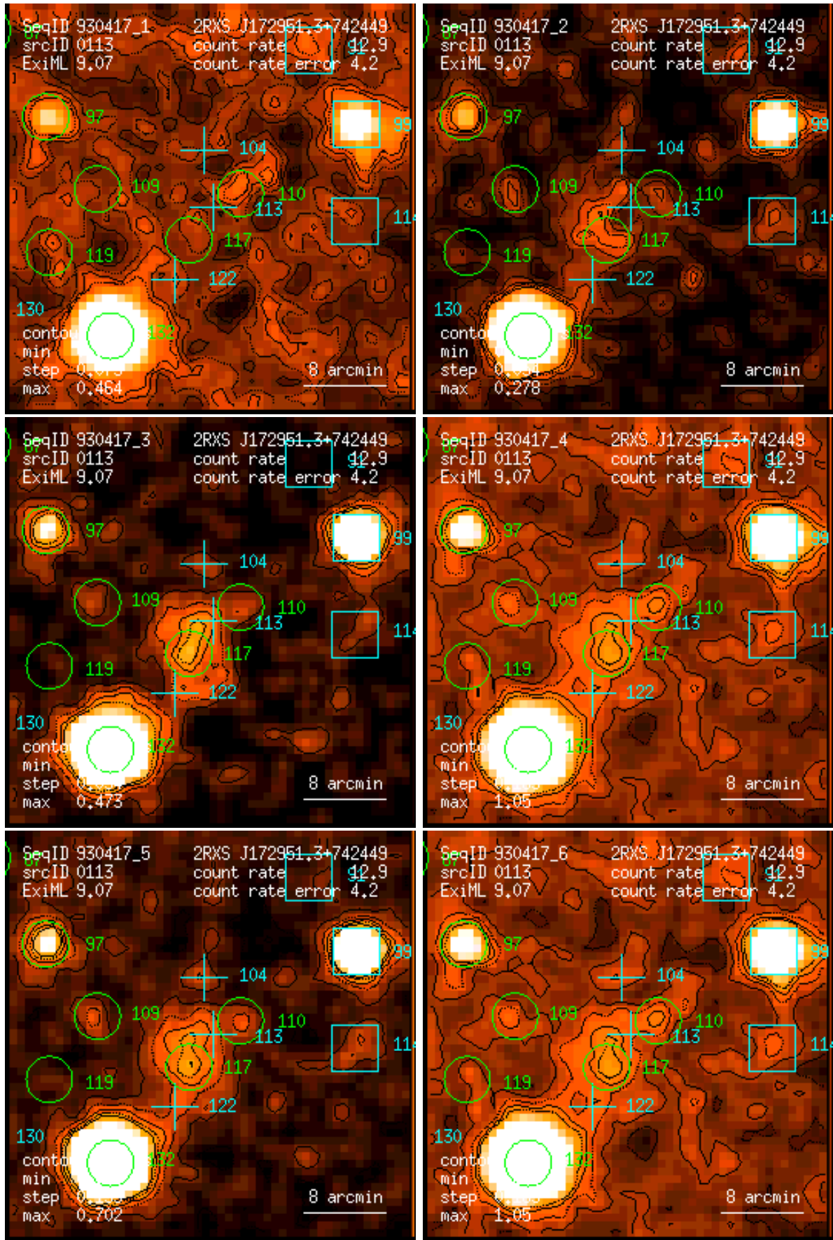
Figure 113: RASS 930417: detection 0113: band rate images, Gaussian filter: (1) PSPC channels 11 – 41, (2) 52 – 90, (3) 91 – 201, (4) 11 – 235, (5) 52 – 201, (6) 11 – 201. Broad band rates in counts/ks. Band rate contour levels in counts/ks/arcmin 2 .
