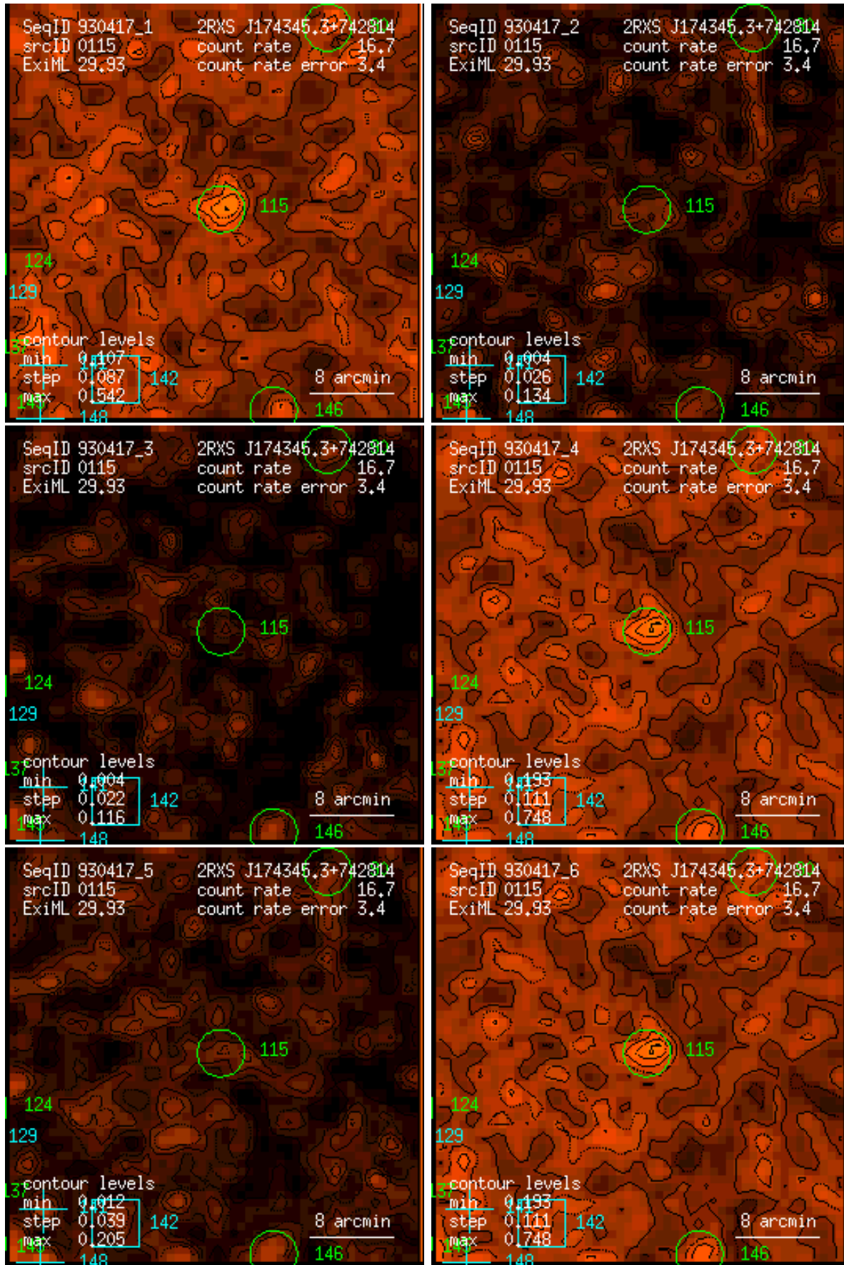
Figure 115: RASS 930417: detection 0115: band rate images, Gaussian filter: (1) PSPC channels 11 – 41, (2) 52 – 90, (3) 91 – 201, (4) 11 – 235, (5) 52 – 201, (6) 11 – 201. Broad band rates in counts/ks. Band rate contour levels in counts/ks/arcmin 2 .
