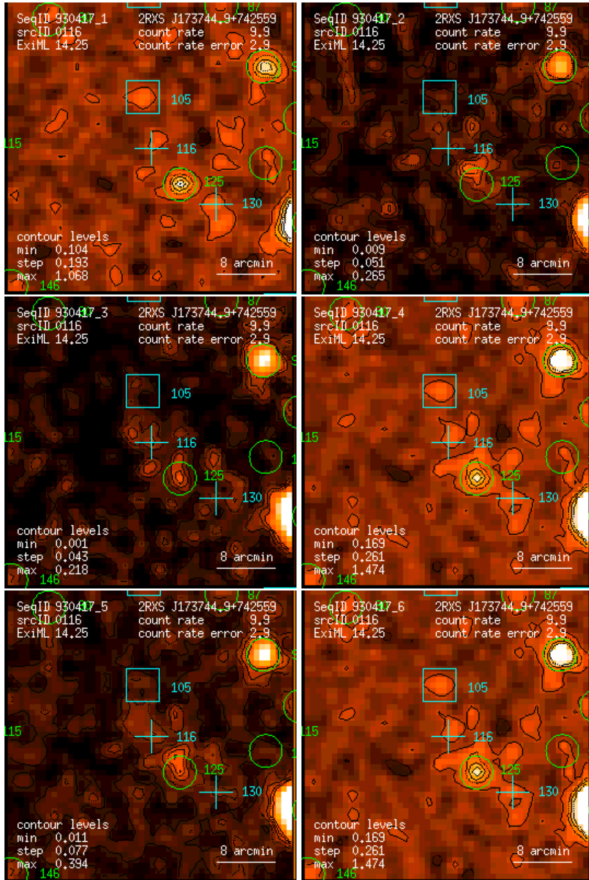
Figure 116: RASS 930417: detection 0116: band rate images, Gaussian filter: (1) PSPC channels 11 – 41, (2) 52 – 90, (3) 91 – 201, (4) 11 – 235, (5) 52 – 201, (6) 11 – 201. Broad band rates in counts/ks. Band rate contour levels in counts/ks/arcmin 2 .
