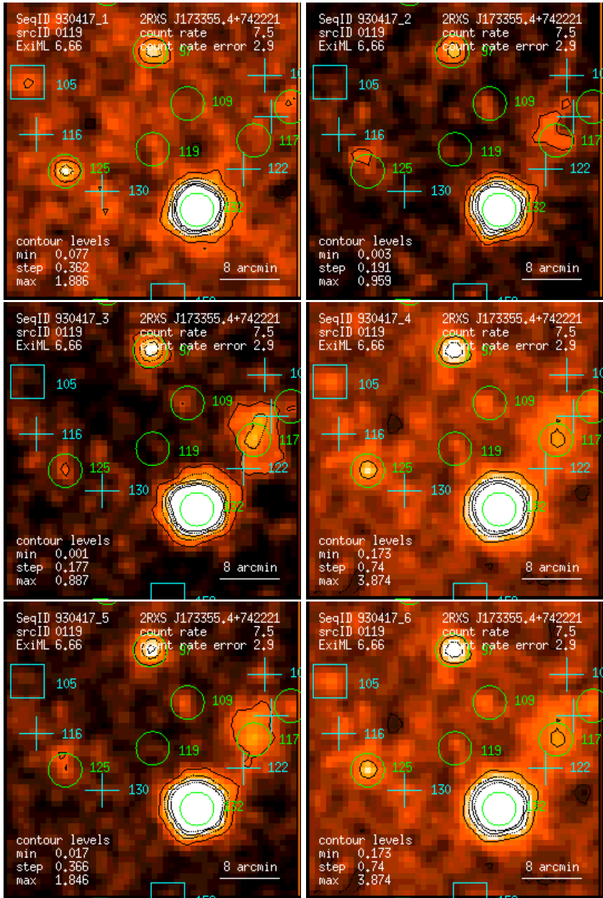
Figure 119: RASS 930417: detection 0119: band rate images, Gaussian filter: (1) PSPC channels 11 – 41, (2) 52 – 90, (3) 91 – 201, (4) 11 – 235, (5) 52 – 201, (6) 11 – 201. Broad band rates in counts/ks. Band rate contour levels in counts/ks/arcmin 2 .
