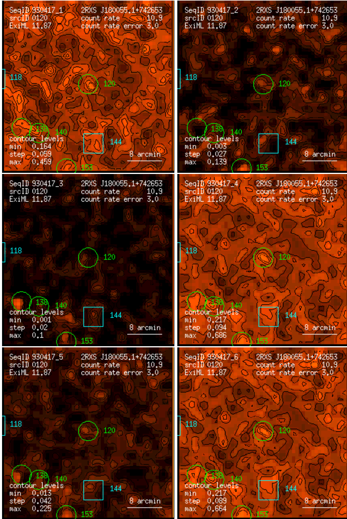
Figure 120: RASS 930417: detection 0120: band rate images, Gaussian filter: (1) PSPC channels 11 – 41, (2) 52 – 90, (3) 91 – 201, (4) 11 – 235, (5) 52 – 201, (6) 11 – 201. Broad band rates in counts/ks. Band rate contour levels in counts/ks/arcmin 2 .
