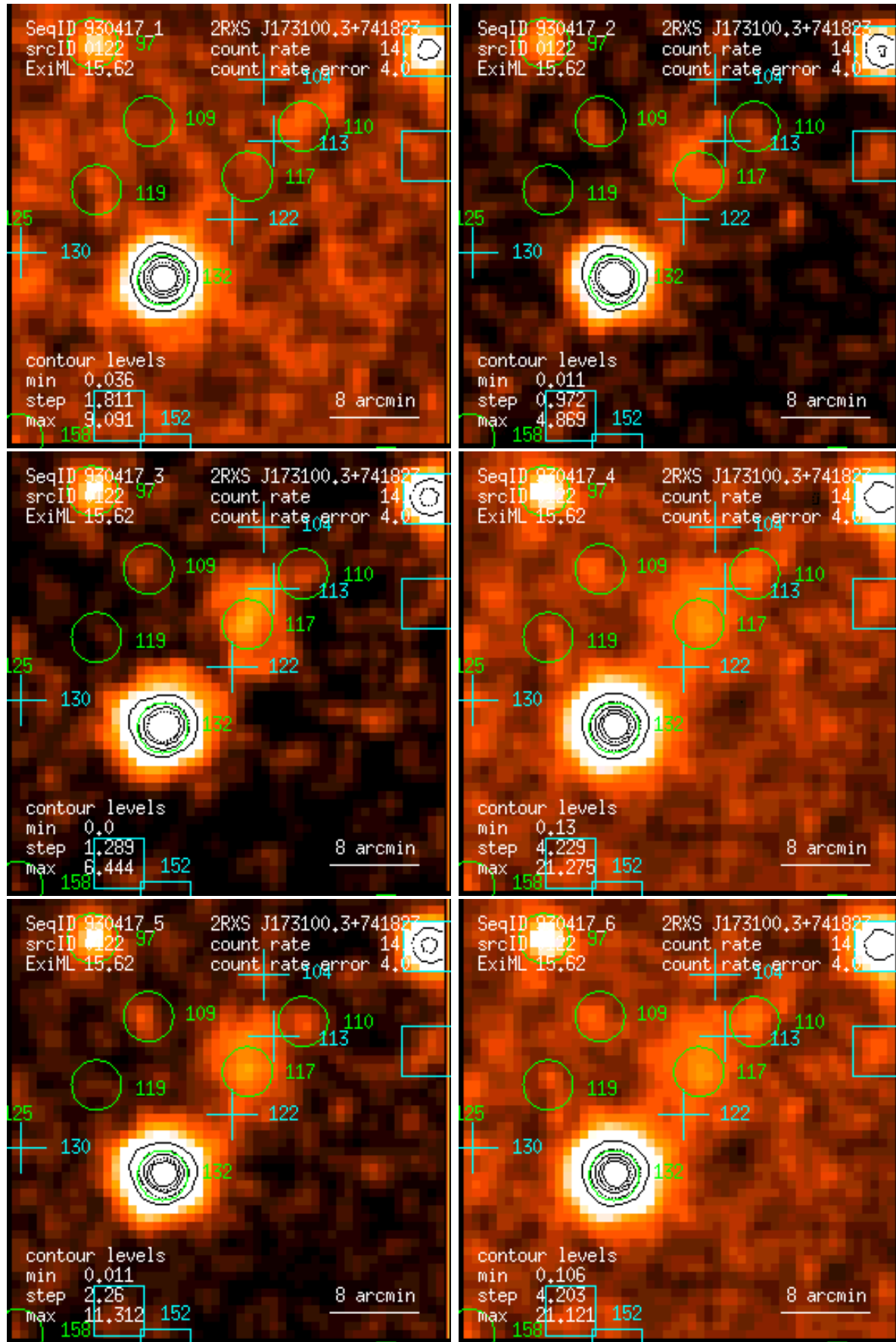
Figure 122: RASS 930417: detection 0122: band rate images, Gaussian filter: (1) PSPC channels 11 – 41, (2) 52 – 90, (3) 91 – 201, (4) 11 – 235, (5) 52 – 201, (6) 11 – 201. Broad band rates in counts/ks. Band rate contour levels in counts/ks/arcmin 2 .
