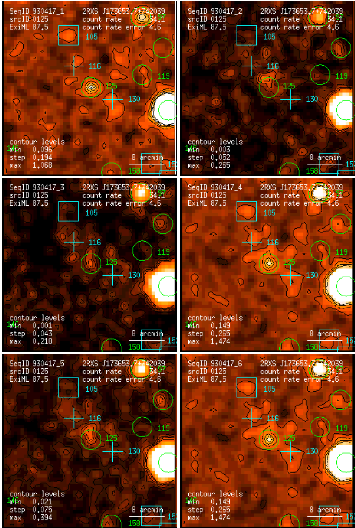
Figure 125: RASS 930417: detection 0125: band rate images, Gaussian filter: (1) PSPC channels 11 – 41, (2) 52 – 90, (3) 91 – 201, (4) 11 – 235, (5) 52 – 201, (6) 11 – 201. Broad band rates in counts/ks. Band rate contour levels in counts/ks/arcmin 2 .
