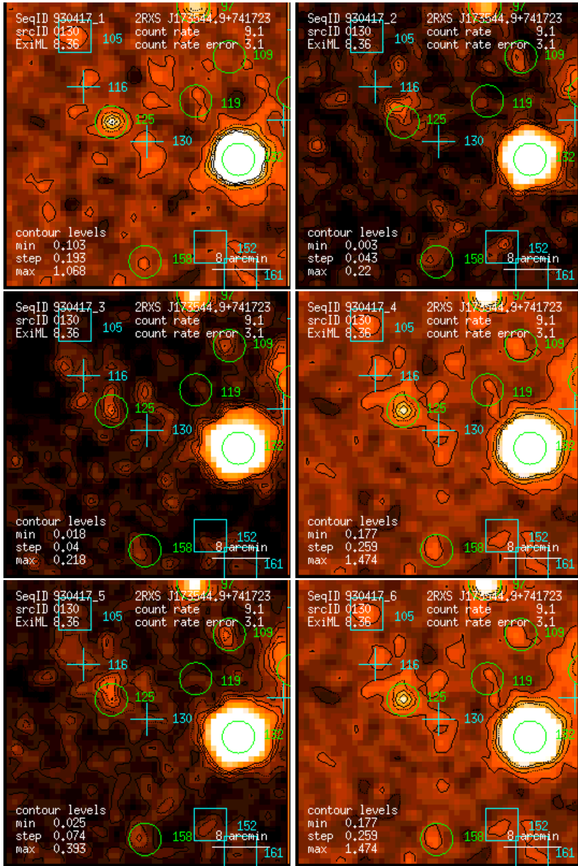
Figure 130: RASS 930417: detection 0130: band rate images, Gaussian filter: (1) PSPC channels 11 – 41, (2) 52 – 90, (3) 91 – 201, (4) 11 – 235, (5) 52 – 201, (6) 11 – 201. Broad band rates in counts/ks. Band rate contour levels in counts/ks/arcmin 2 .
