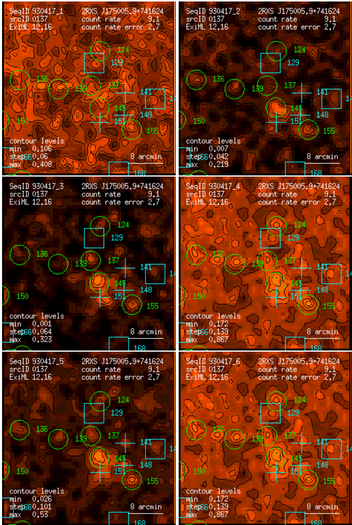
Figure 137: RASS 930417: detection 0137: band rate images, Gaussian filter: (1) PSPC channels 11 – 41, (2) 52 – 90, (3) 91 – 201, (4) 11 – 235, (5) 52 – 201, (6) 11 – 201. Broad band rates in counts/ks. Band rate contour levels in counts/ks/arcmin 2 .
