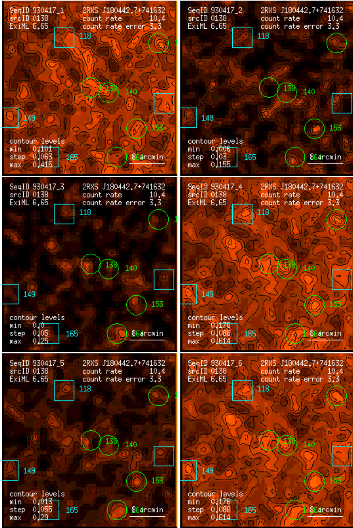
Figure 138: RASS 930417: detection 0138: band rate images, Gaussian filter: (1) PSPC channels 11 – 41, (2) 52 – 90, (3) 91 – 201, (4) 11 – 235, (5) 52 – 201, (6) 11 – 201. Broad band rates in counts/ks. Band rate contour levels in counts/ks/arcmin 2 .
