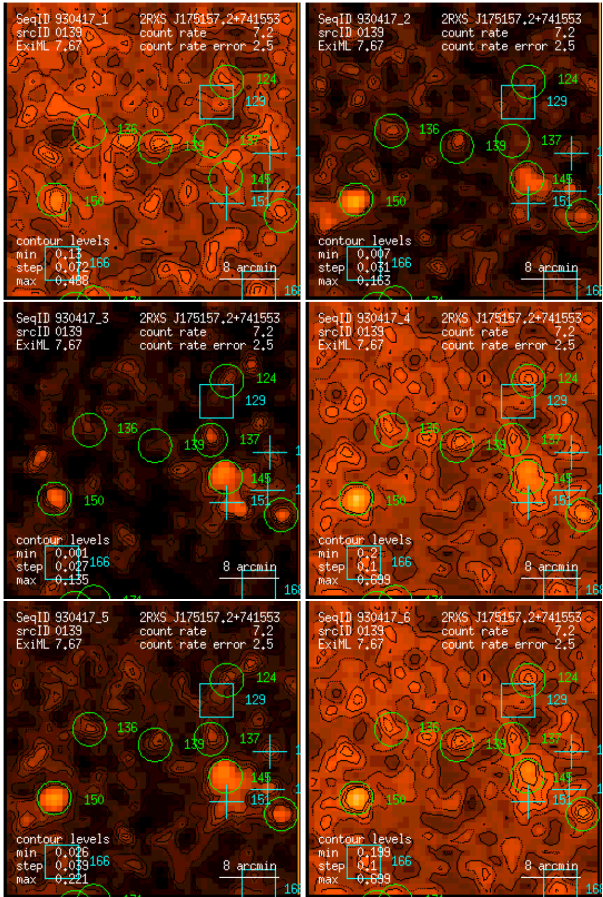
Figure 139: RASS 930417: detection 0139: band rate images, Gaussian filter: (1) PSPC channels 11 – 41, (2) 52 – 90, (3) 91 – 201, (4) 11 – 235, (5) 52 – 201, (6) 11 – 201. Broad band rates in counts/ks. Band rate contour levels in counts/ks/arcmin 2 .
