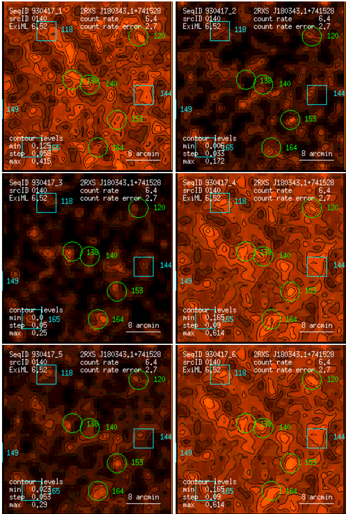
Figure 140: RASS 930417: detection 0140: band rate images, Gaussian filter: (1) PSPC channels 11 – 41, (2) 52 – 90, (3) 91 – 201, (4) 11 – 235, (5) 52 – 201, (6) 11 – 201. Broad band rates in counts/ks. Band rate contour levels in counts/ks/arcmin 2 .
