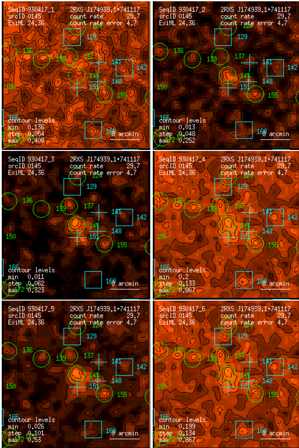
Figure 145: RASS 930417: detection 0145: band rate images, Gaussian filter: (1) PSPC channels 11 – 41, (2) 52 – 90, (3) 91 – 201, (4) 11 – 235, (5) 52 – 201, (6) 11 – 201. Broad band rates in counts/ks. Band rate contour levels in counts/ks/arcmin 2 .
