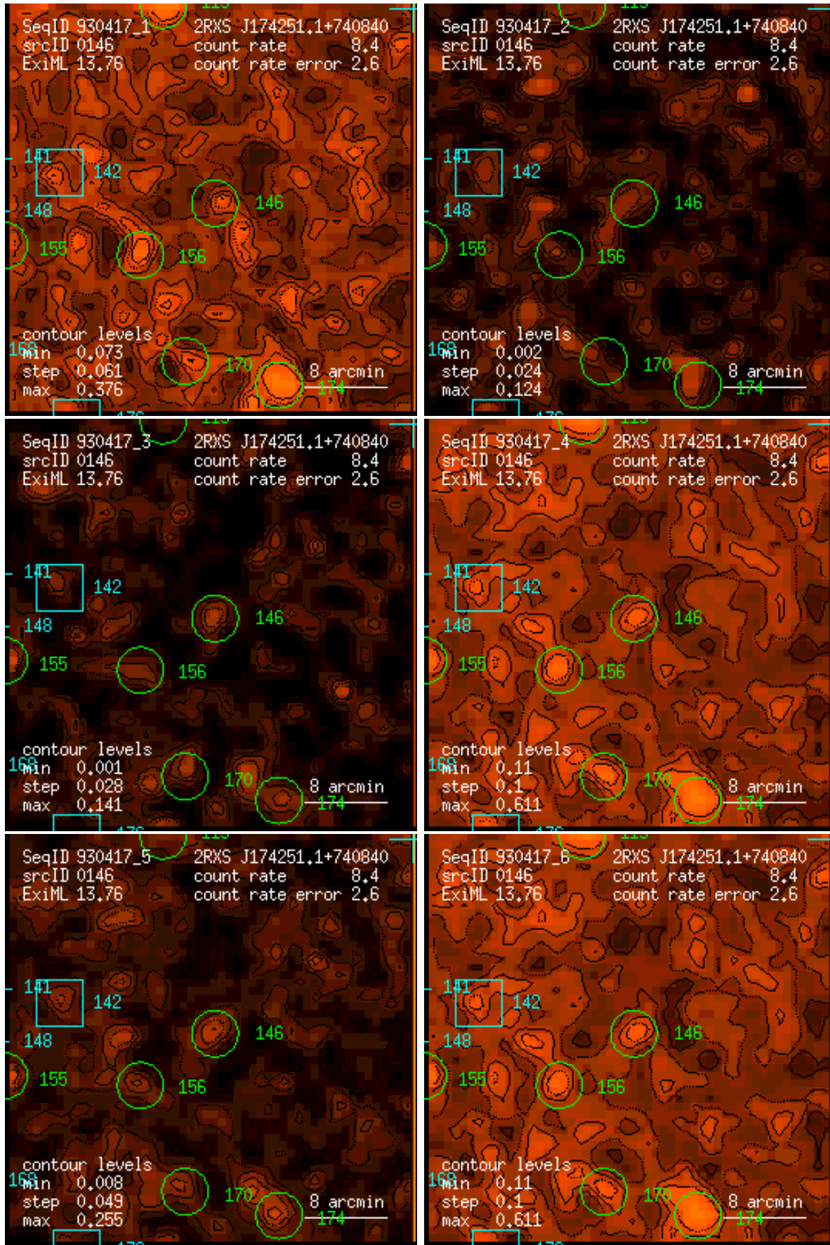
Figure 146: RASS 930417: detection 0146: band rate images, Gaussian filter: (1) PSPC channels 11 – 41, (2) 52 – 90, (3) 91 – 201, (4) 11 – 235, (5) 52 – 201, (6) 11 – 201. Broad band rates in counts/ks. Band rate contour levels in counts/ks/arcmin 2 .
