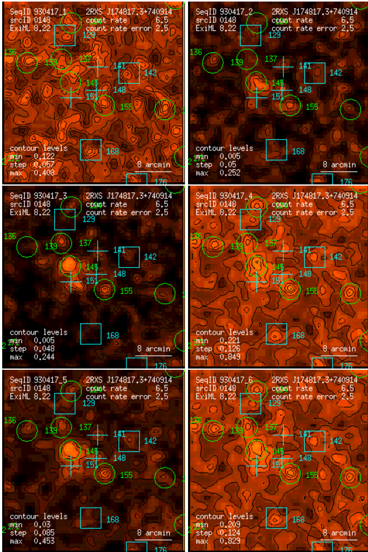
Figure 148: RASS 930417: detection 0148: band rate images, Gaussian filter: (1) PSPC channels 11 – 41, (2) 52 – 90, (3) 91 – 201, (4) 11 – 235, (5) 52 – 201, (6) 11 – 201. Broad band rates in counts/ks. Band rate contour levels in counts/ks/arcmin 2 .
