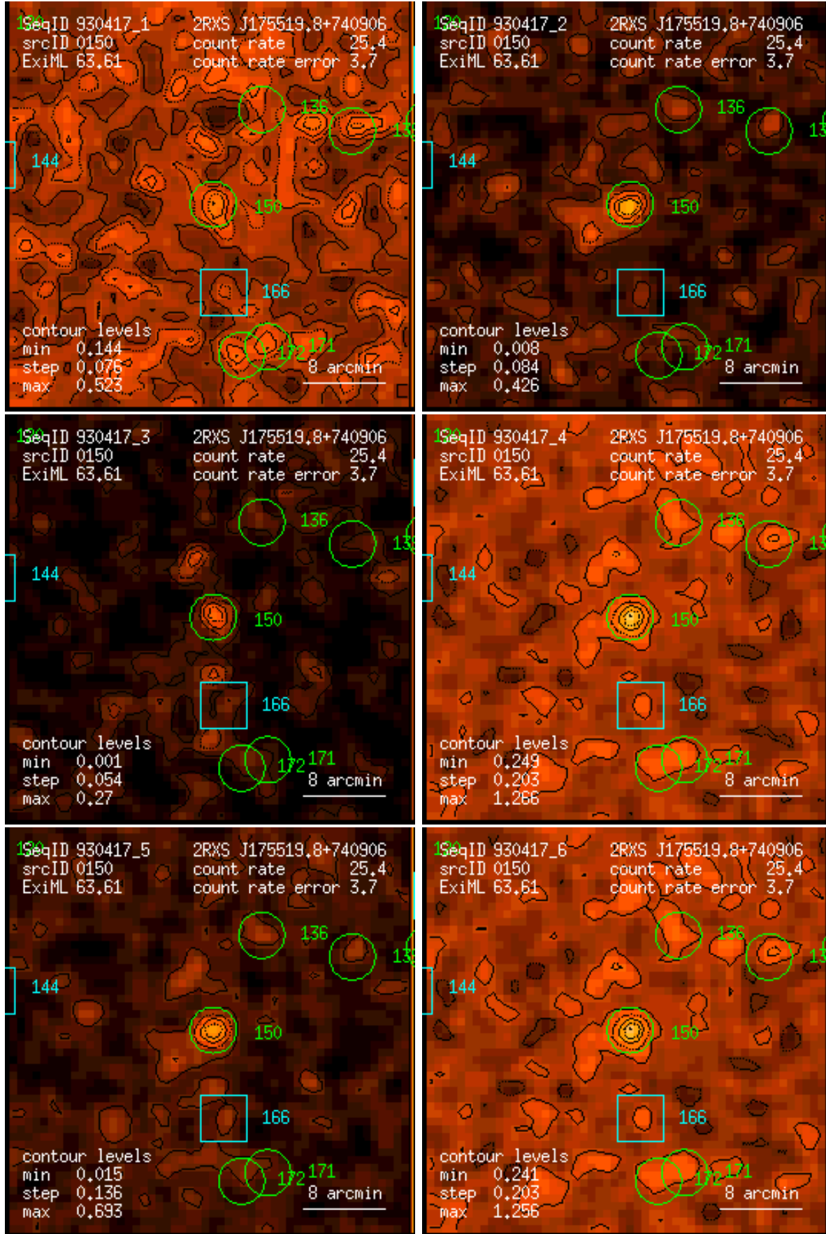
Figure 150: RASS 930417: detection 0150: band rate images, Gaussian filter: (1) PSPC channels 11 – 41, (2) 52 – 90, (3) 91 – 201, (4) 11 – 235, (5) 52 – 201, (6) 11 – 201. Broad band rates in counts/ks. Band rate contour levels in counts/ks/arcmin 2 .
