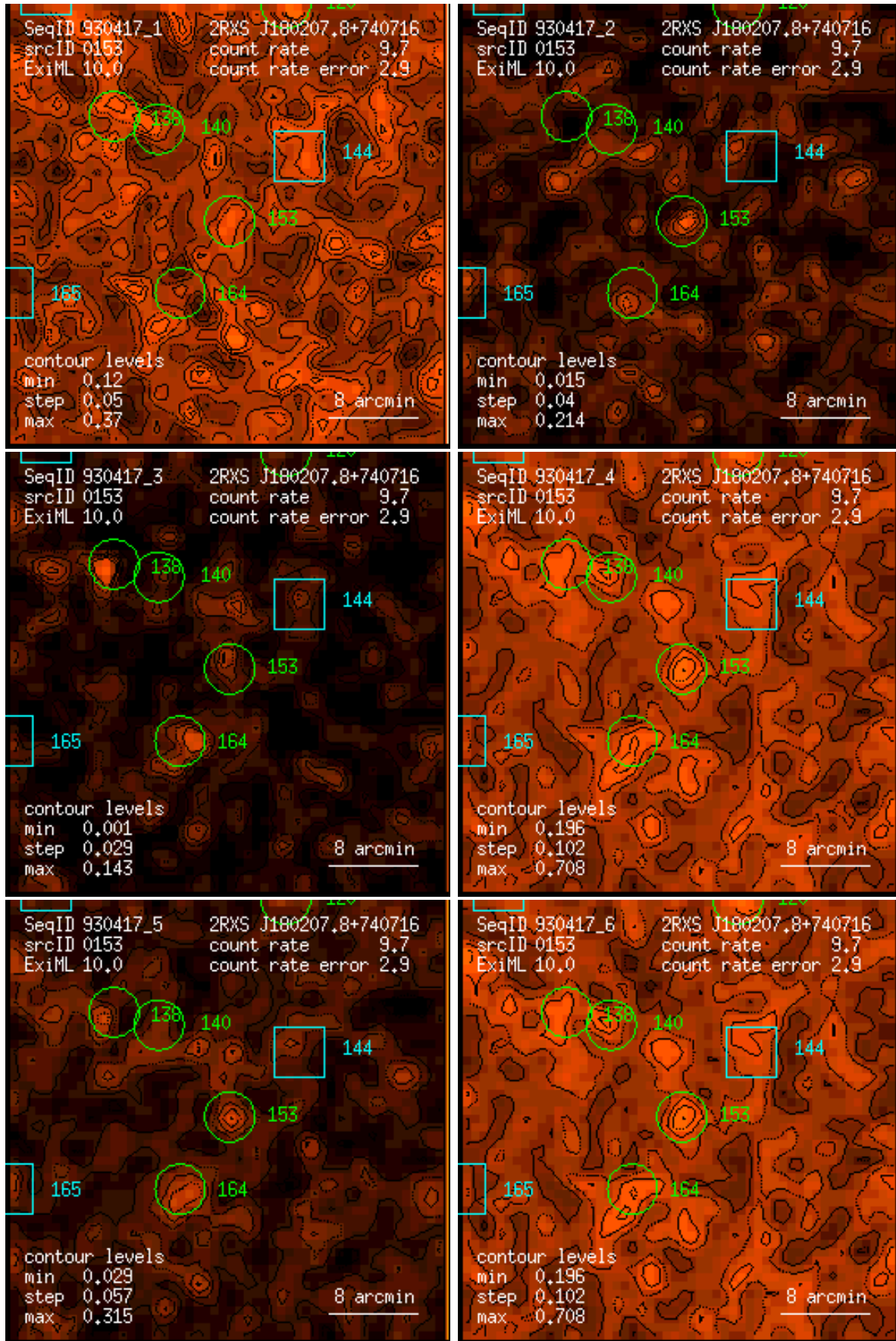
Figure 153: RASS 930417: detection 0153: band rate images, Gaussian filter: (1) PSPC channels 11 – 41, (2) 52 – 90, (3) 91 – 201, (4) 11 – 235, (5) 52 – 201, (6) 11 – 201. Broad band rates in counts/ks. Band rate contour levels in counts/ks/arcmin 2 .
