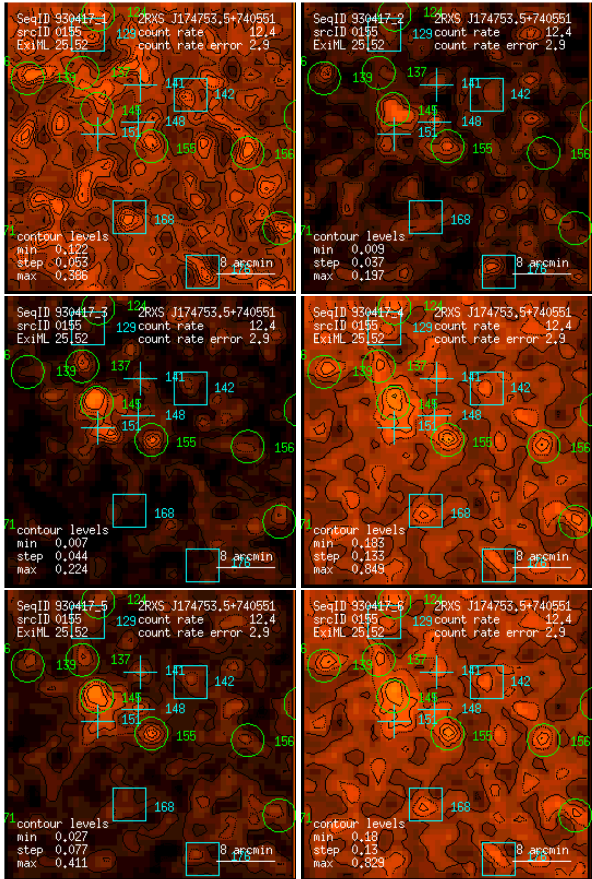
Figure 155: RASS 930417: detection 0155: band rate images, Gaussian filter: (1) PSPC channels 11 – 41, (2) 52 – 90, (3) 91 – 201, (4) 11 – 235, (5) 52 – 201, (6) 11 – 201. Broad band rates in counts/ks. Band rate contour levels in counts/ks/arcmin 2 .
