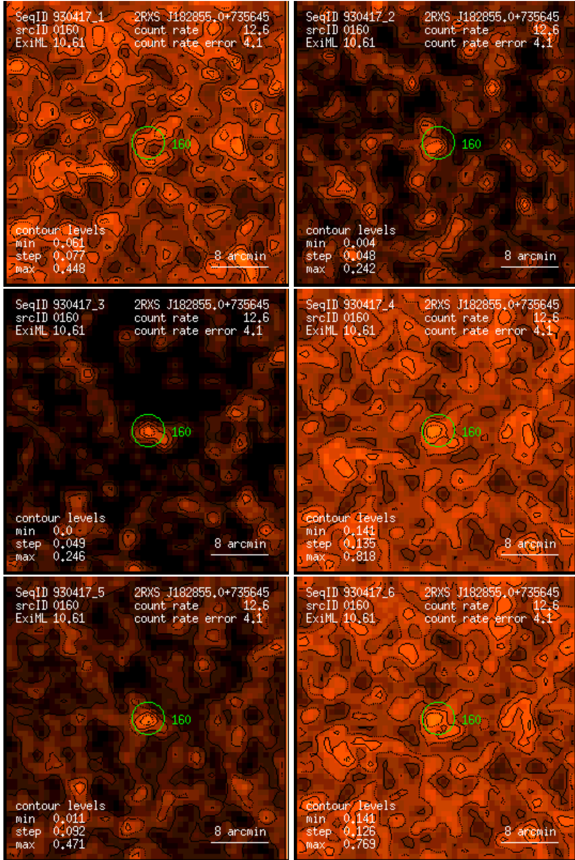
Figure 160: RASS 930417: detection 0160: band rate images, Gaussian filter: (1) PSPC channels 11 – 41, (2) 52 – 90, (3) 91 – 201, (4) 11 – 235, (5) 52 – 201, (6) 11 – 201. Broad band rates in counts/ks. Band rate contour levels in counts/ks/arcmin 2 .
